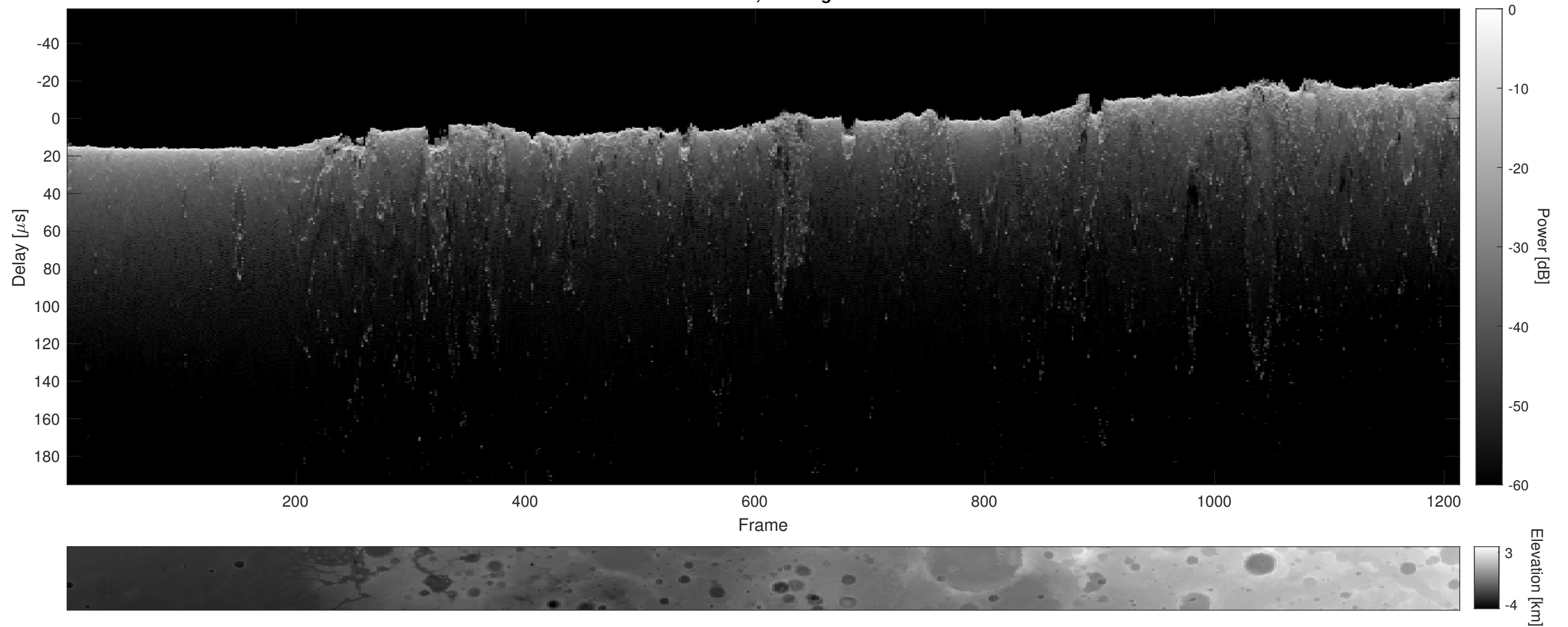
Orbit 21911, Cluttergram
