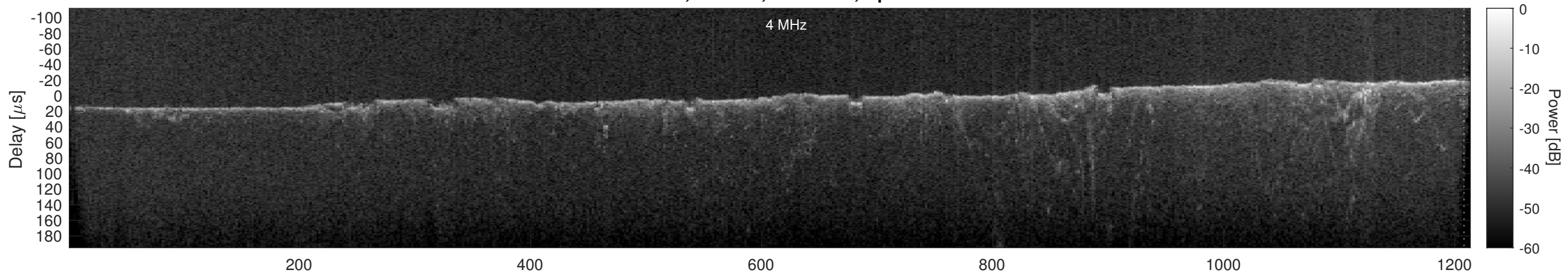
Orbit 21911, Cluttergram
