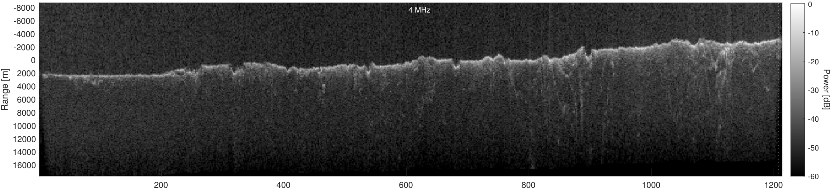
Orbit 21911, Depth-Corrected Cluttergram
