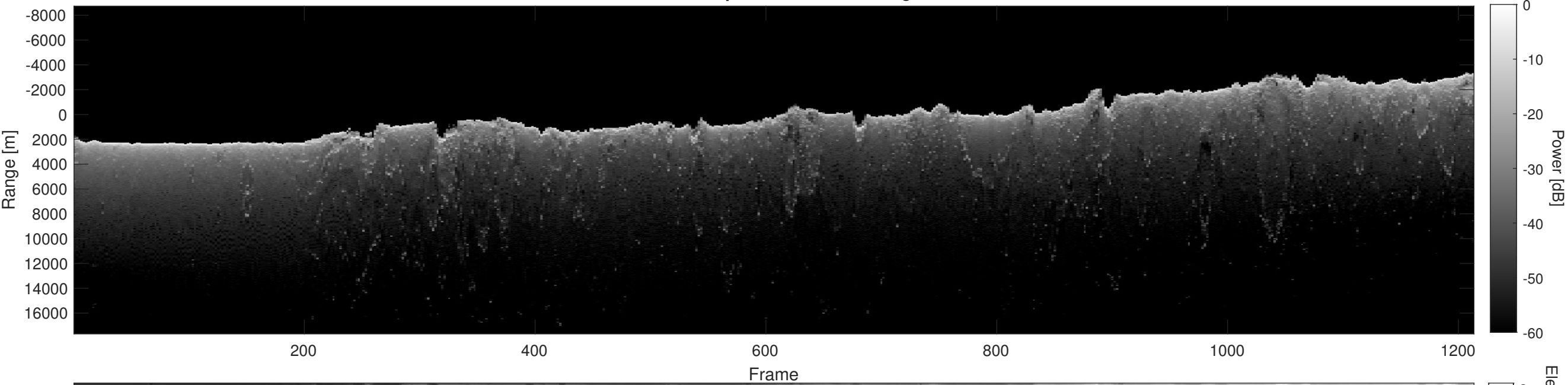
Orbit 21911, Depth-Corrected Cluttergram
