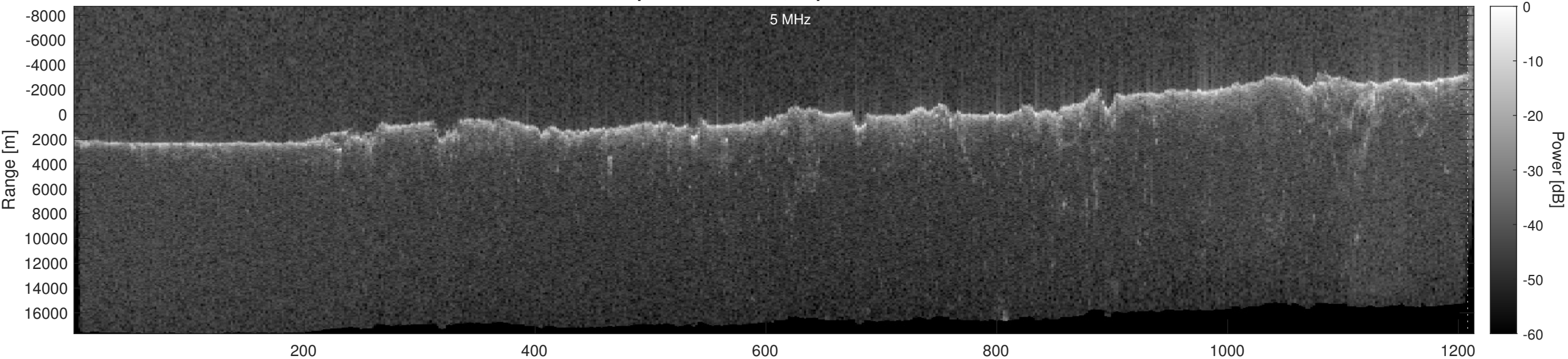
Orbit 21911, Optimized, Window, Depth-Corrected, Channel 2
