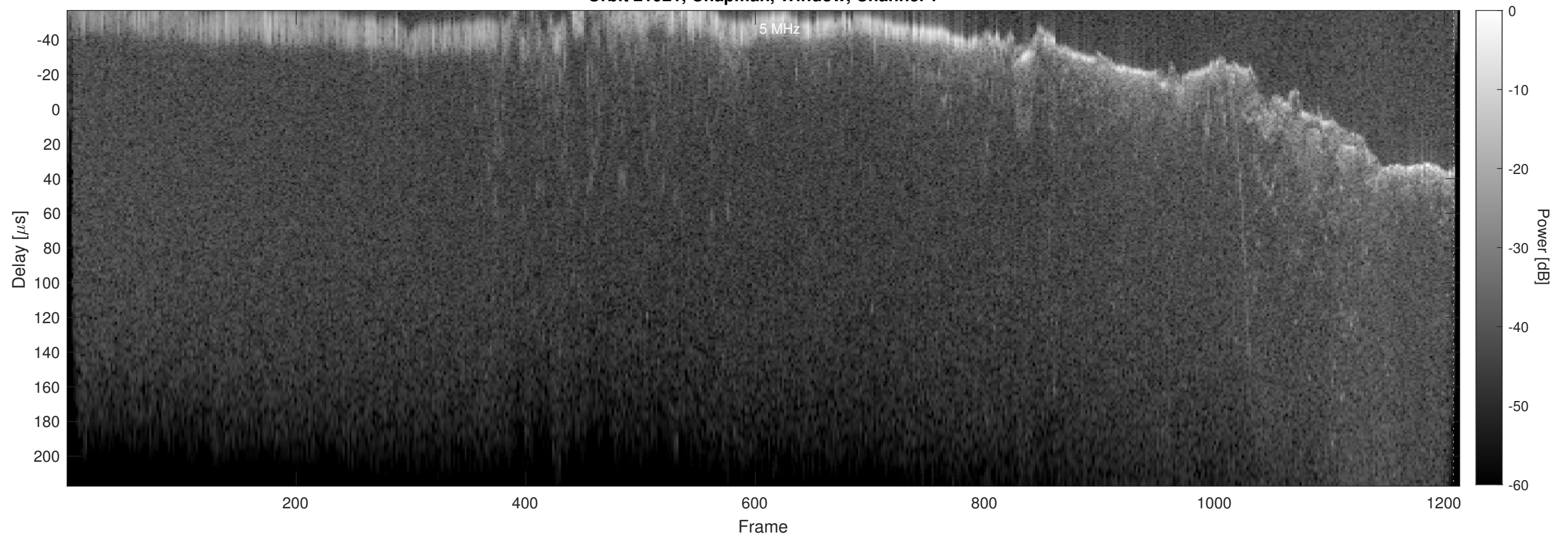
Orbit 21921, Chapman, Window, Channel 2
