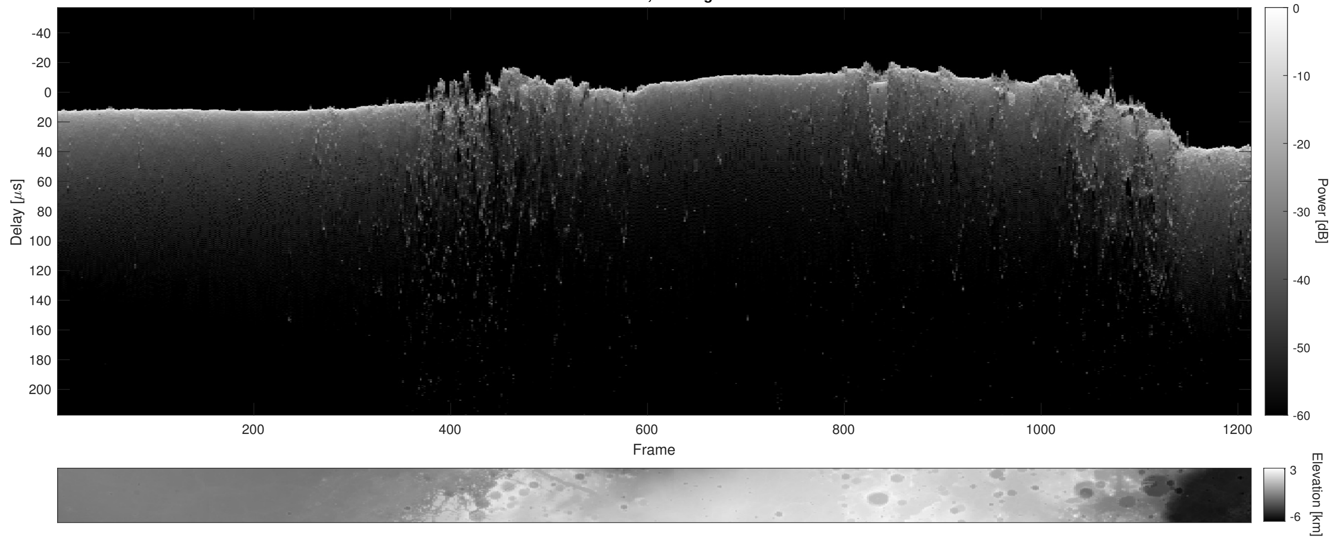
Orbit 21921, Cluttergram
