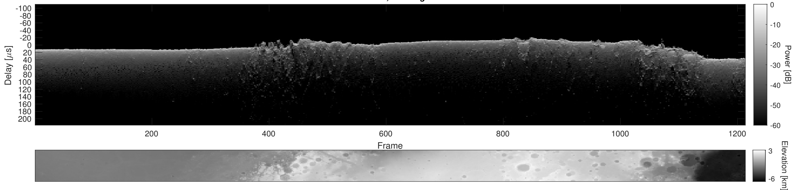
Orbit 21921, Cluttergram
