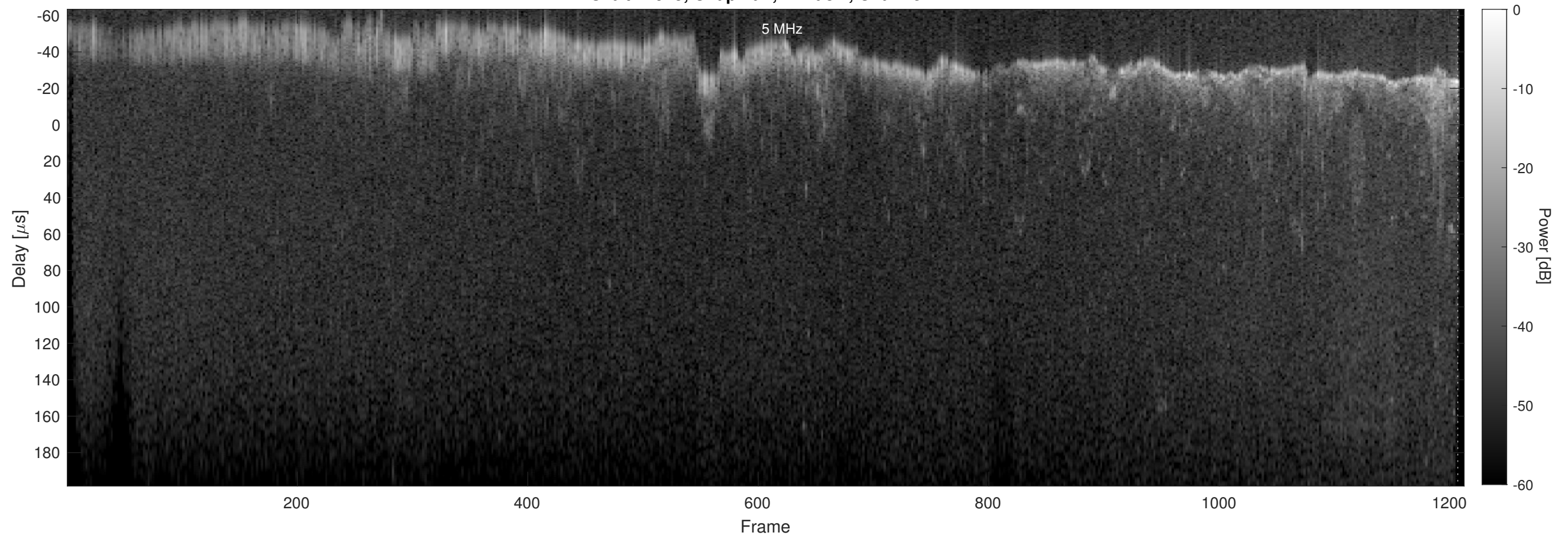
Orbit 21925, Chapman, Window, Channel 2
