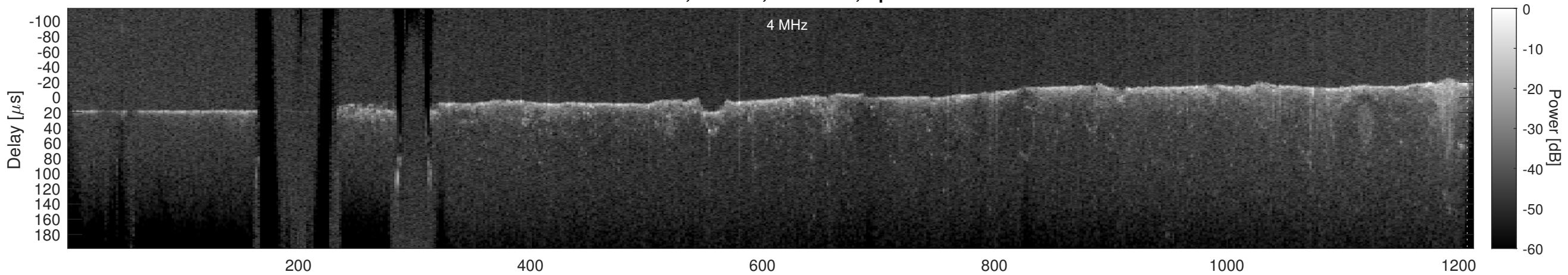
Orbit 21925, Cluttergram
