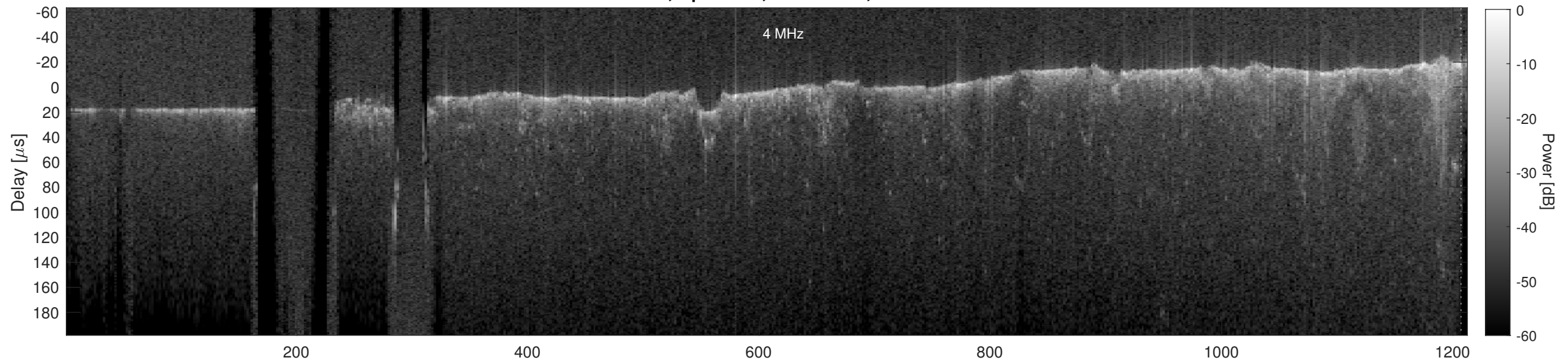
Orbit 21925, Cluttergram
