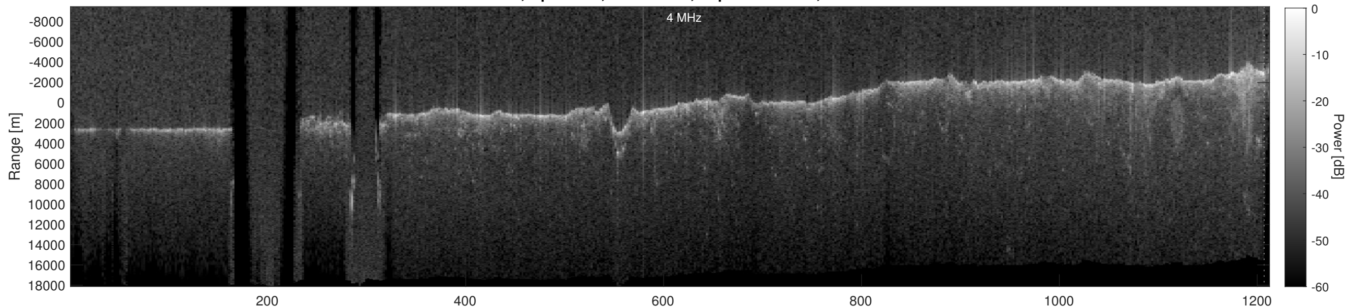
Orbit 21925, Depth-Corrected Cluttergram
