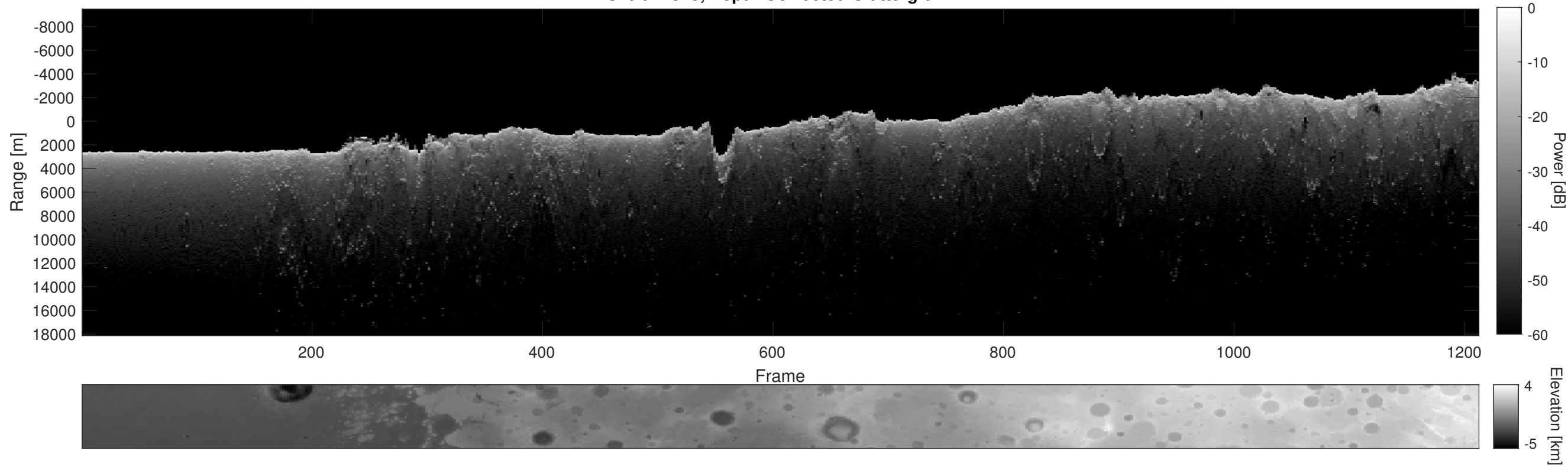
Orbit 21925, Depth-Corrected Cluttergram
