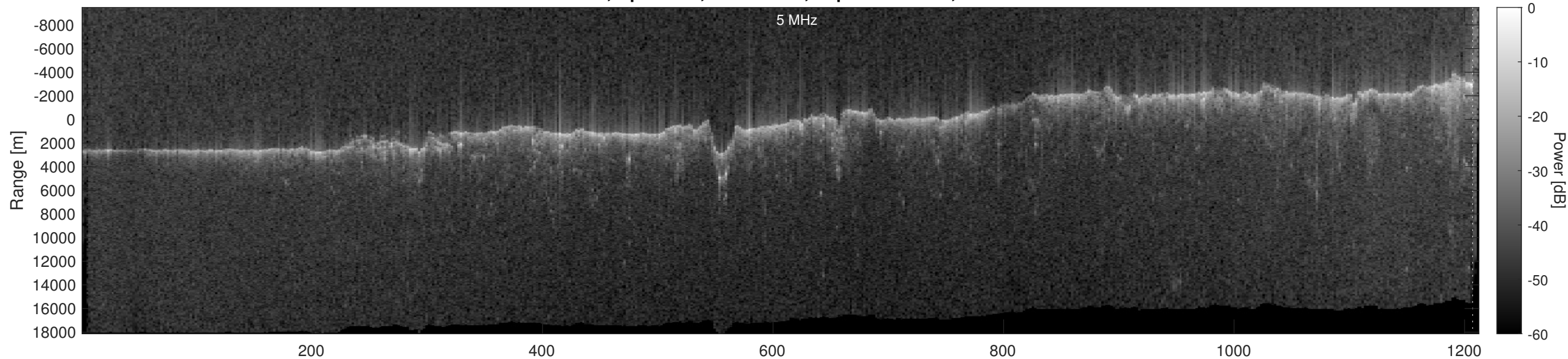
Orbit 21925, Optimized, No Window, Depth-Corrected, Channel 2
