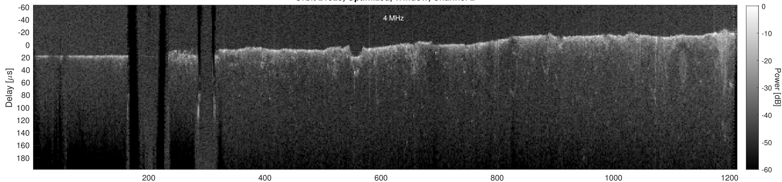
Orbit 21925, Cluttergram
