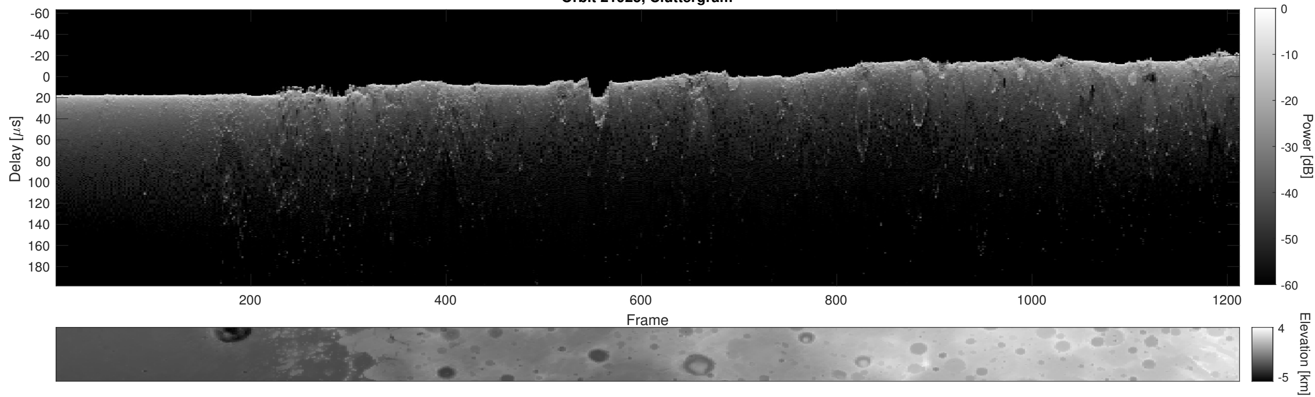
Orbit 21925, Cluttergram
