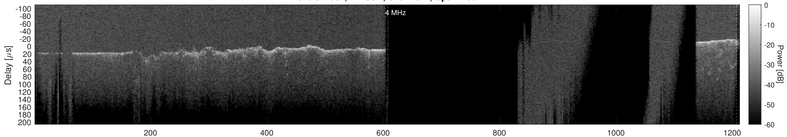
Orbit 21932, Cluttergram
