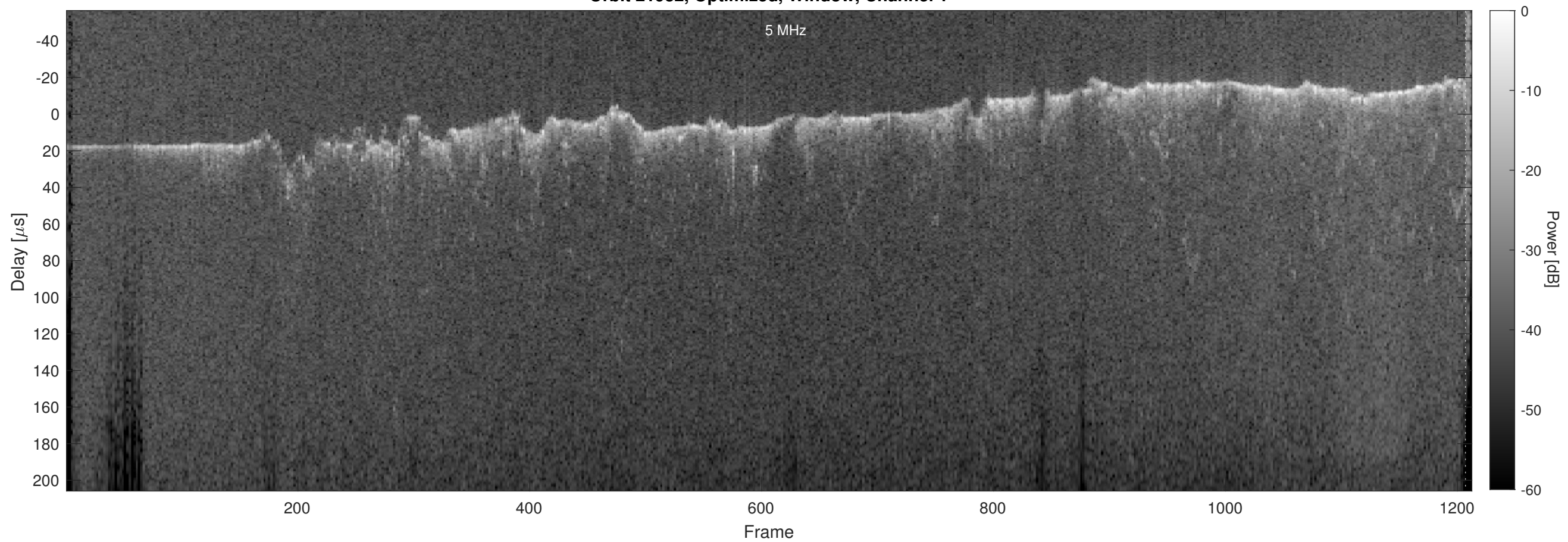
Orbit 21932, Optimized, Window, Channel 2
