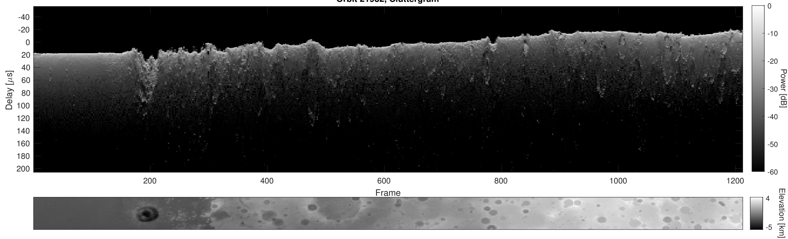
Orbit 21932, Cluttergram
