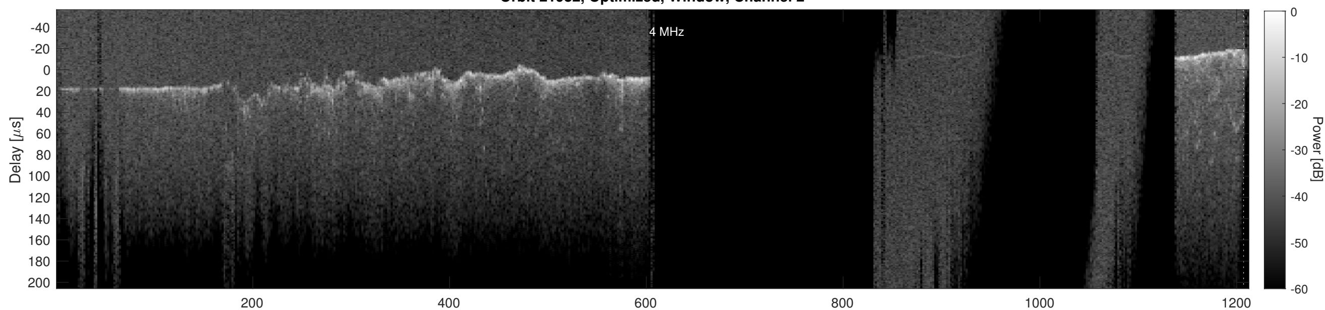
Orbit 21932, Cluttergram
