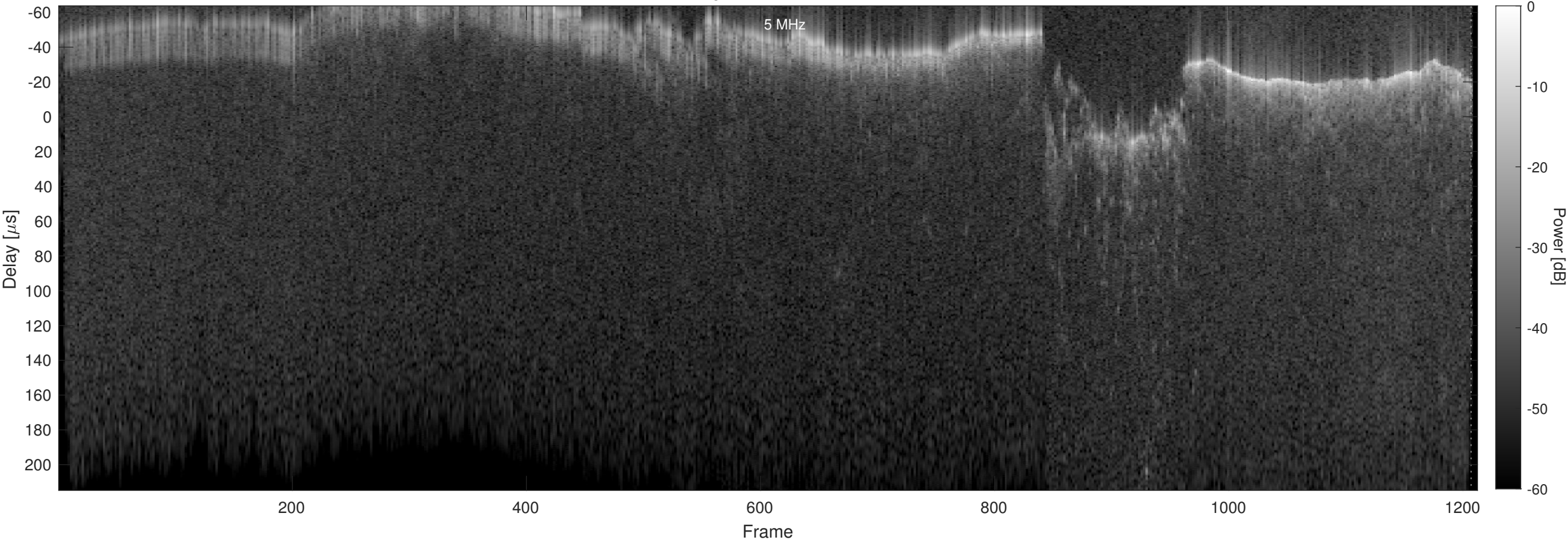
Orbit 21933, Chapman, No Window, Channel 2
