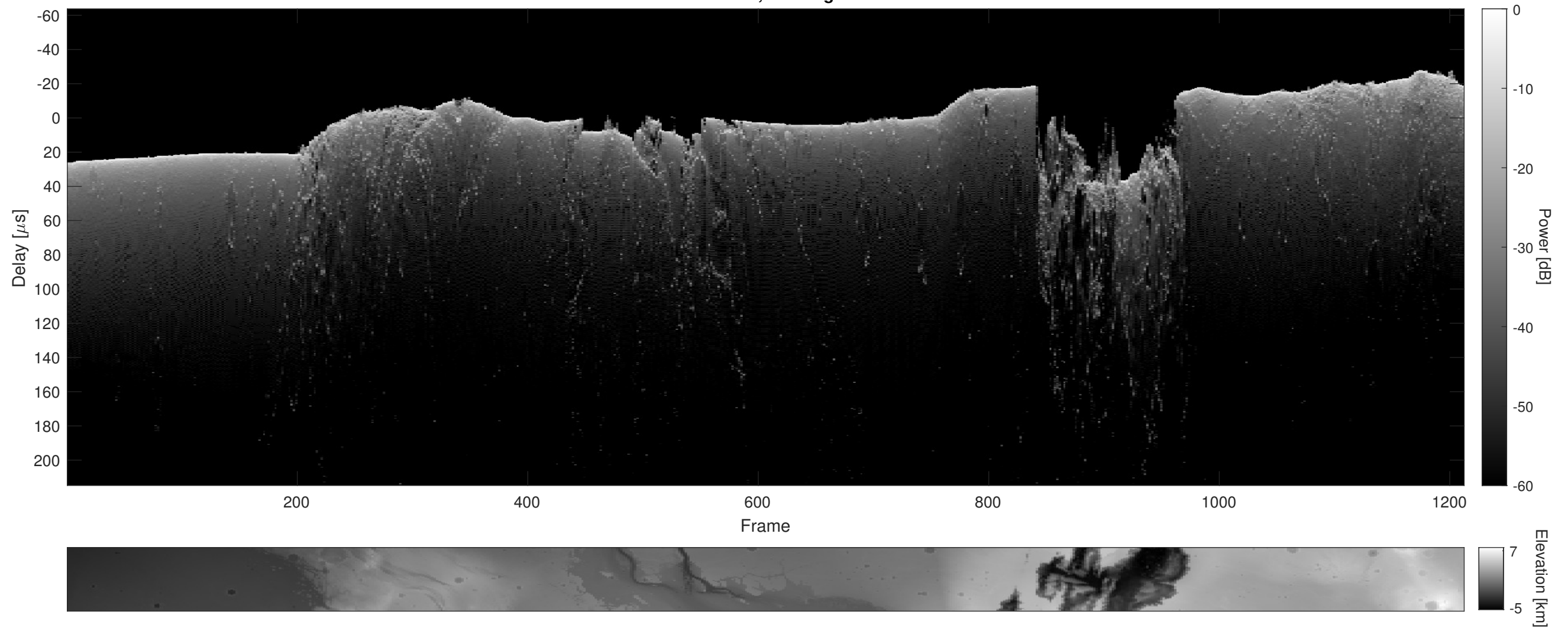
Orbit 21933, Cluttergram
