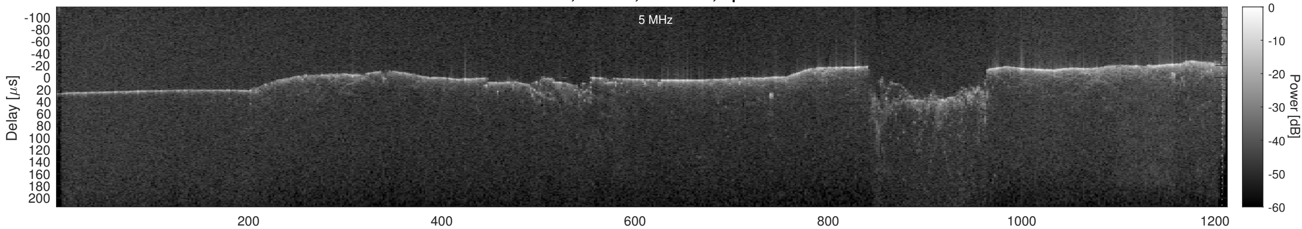
Orbit 21933, Cluttergram
