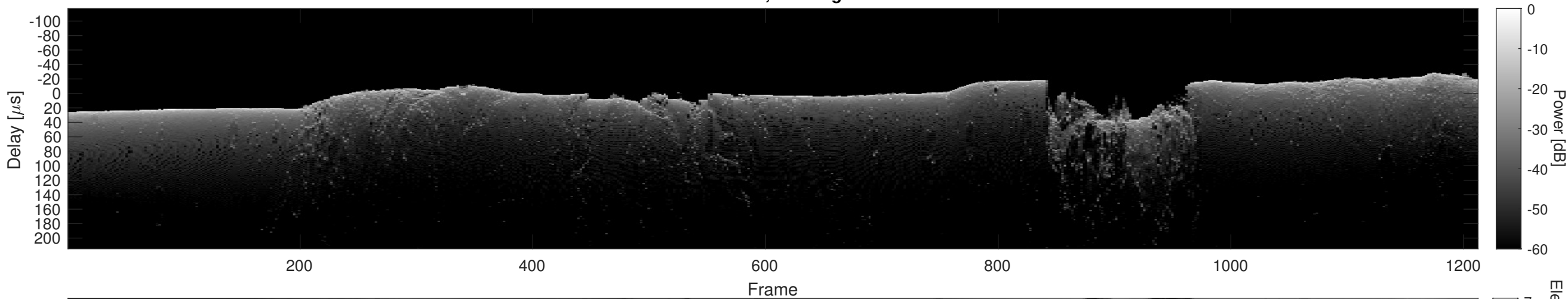
Orbit 21933, Cluttergram
