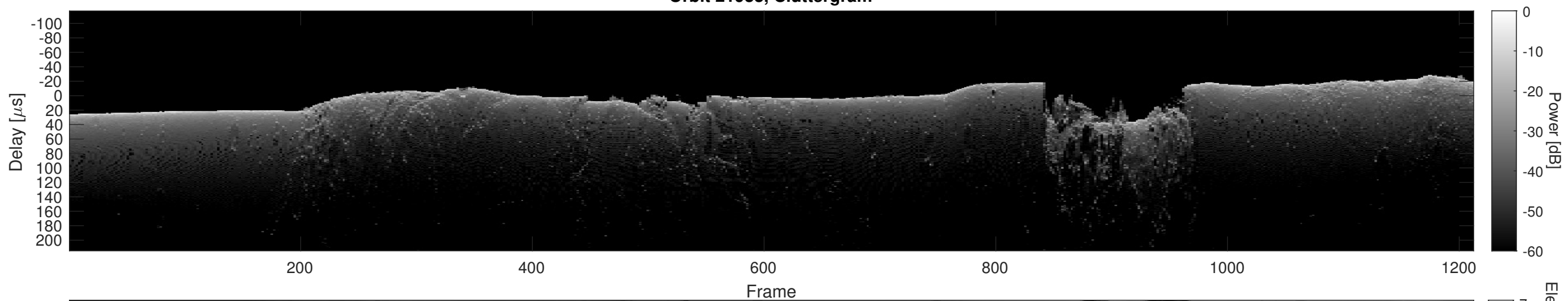
Orbit 21933, Cluttergram
