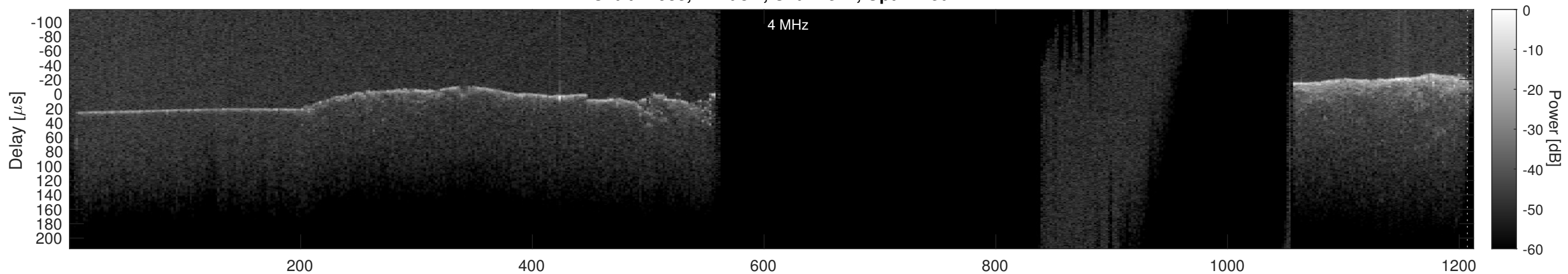
Orbit 21933, Cluttergram
