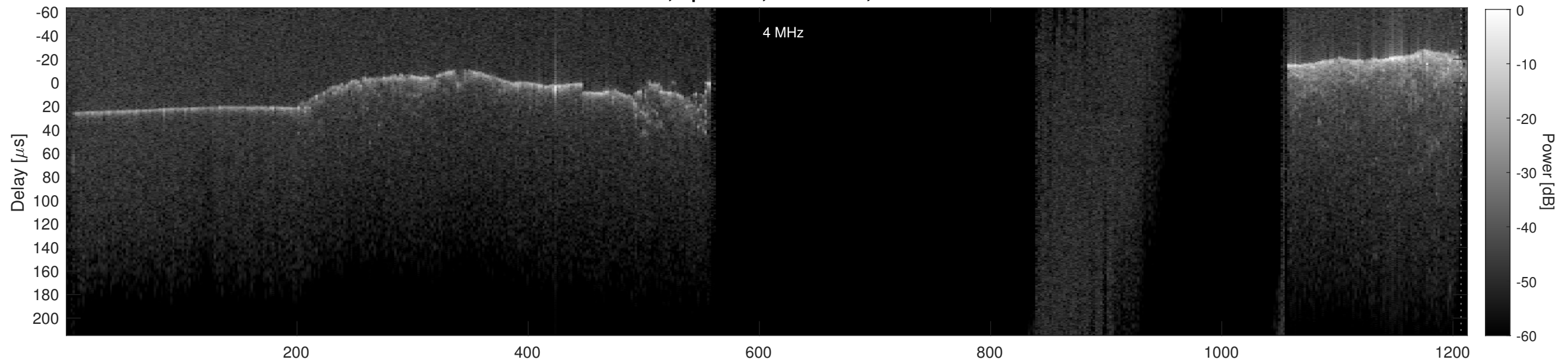
Orbit 21933, Cluttergram
