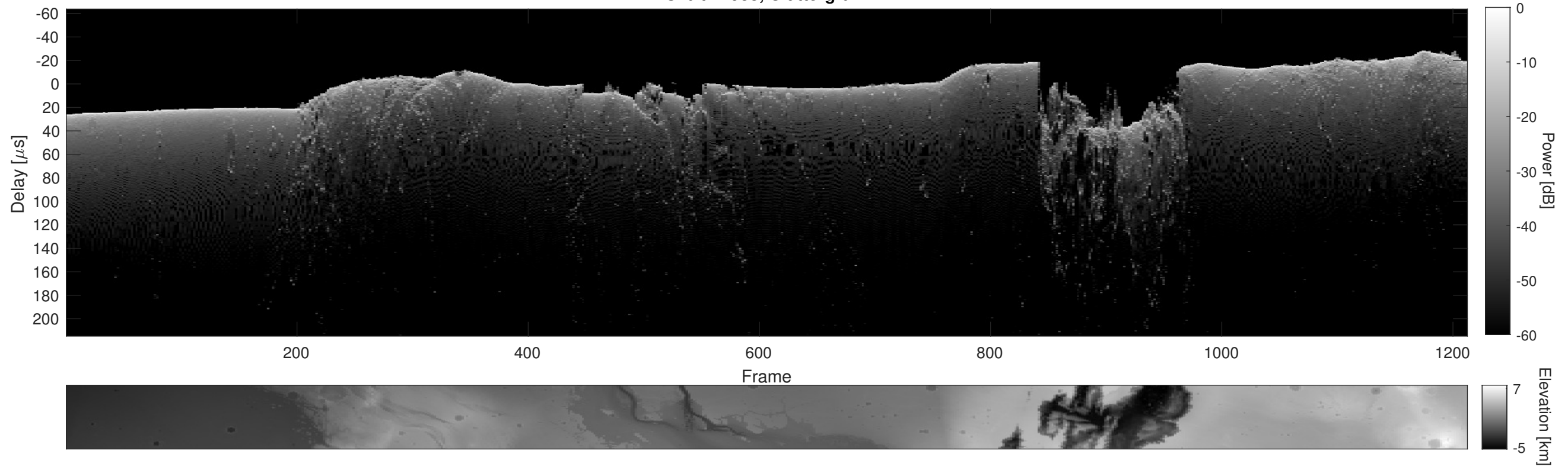
Orbit 21933, Cluttergram
