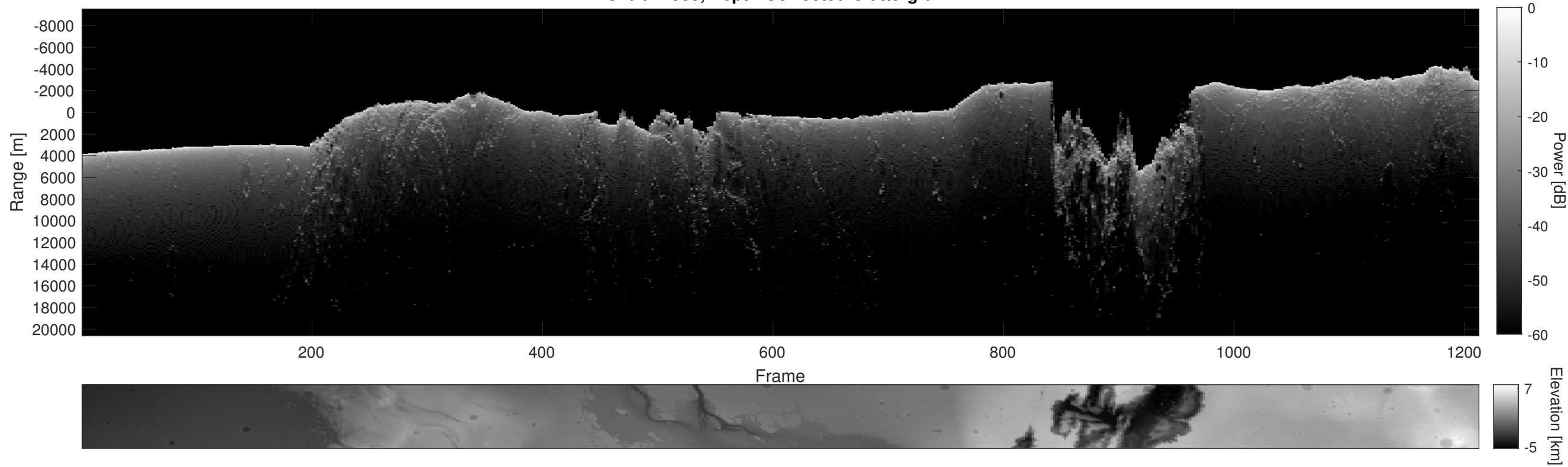
Orbit 21933, Depth-Corrected Cluttergram
