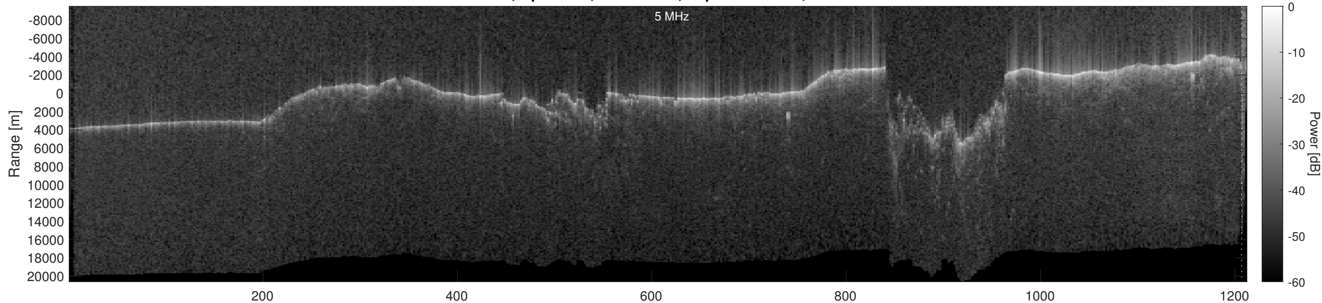
Orbit 21933, Optimized, No Window, Depth-Corrected, Channel 2
