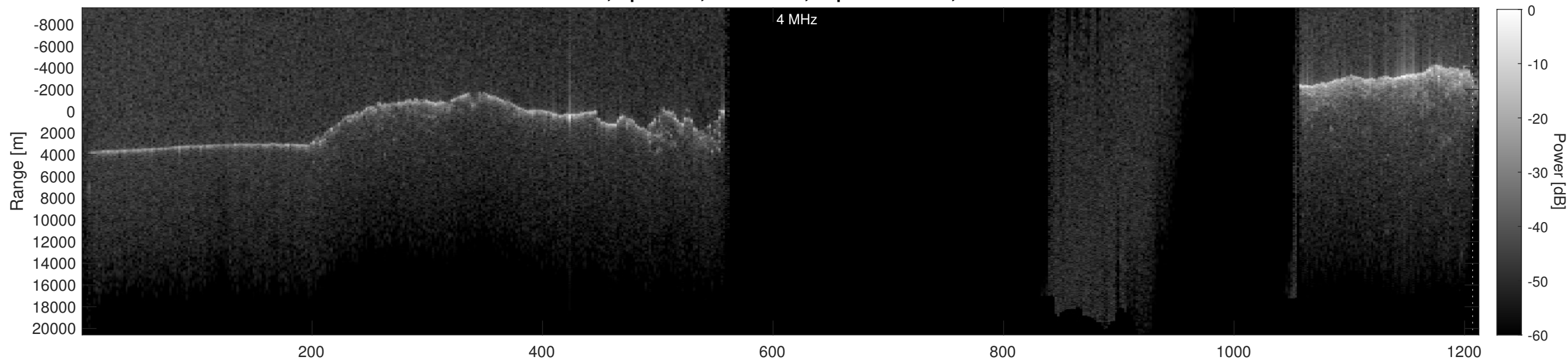
Orbit 21933, Depth-Corrected Cluttergram
