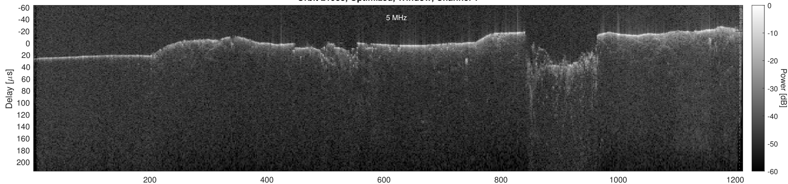
Orbit 21933, Optimized, Window, Channel 2
