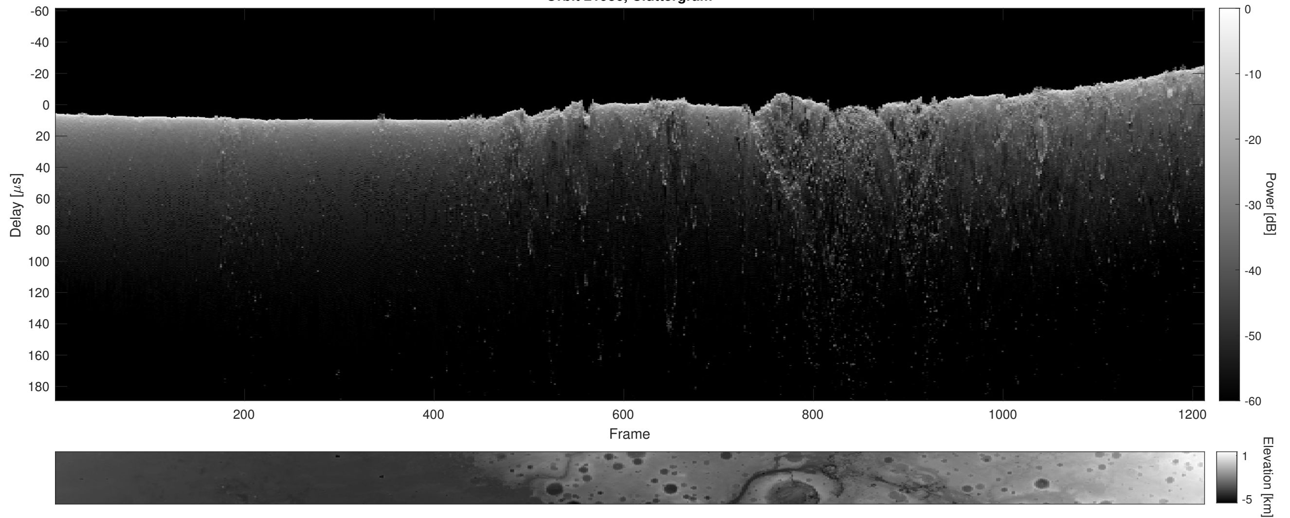
Orbit 21936, Cluttergram
