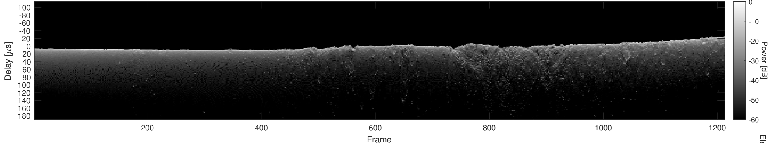
Orbit 21936, Cluttergram
