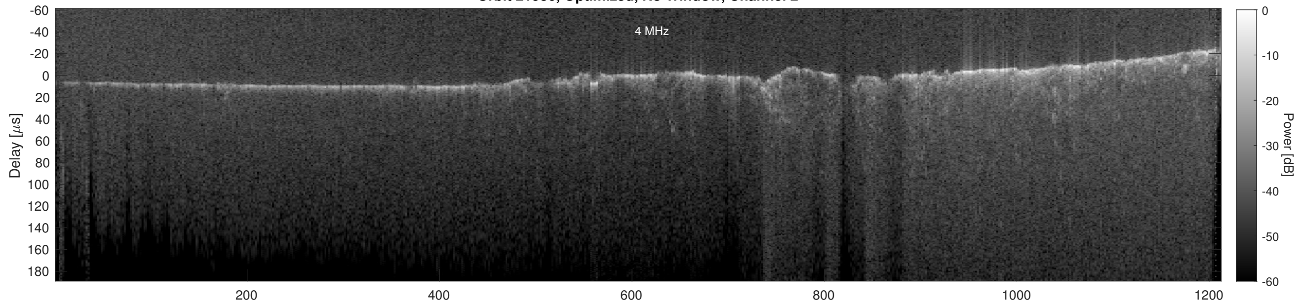
Orbit 21936, Cluttergram
