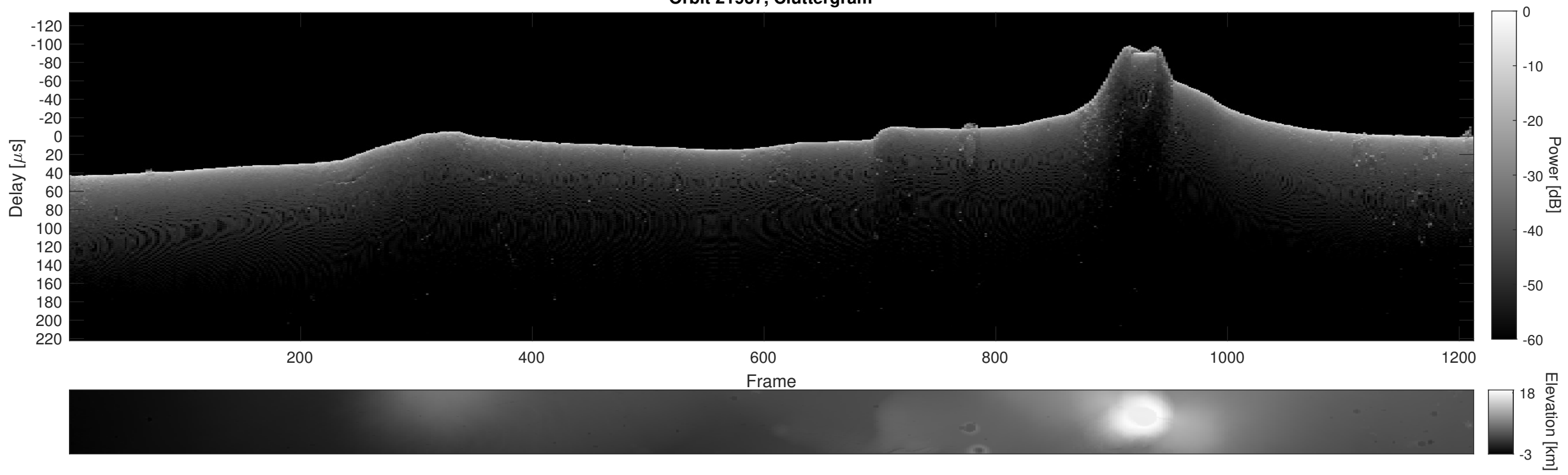
Orbit 21937, Cluttergram
