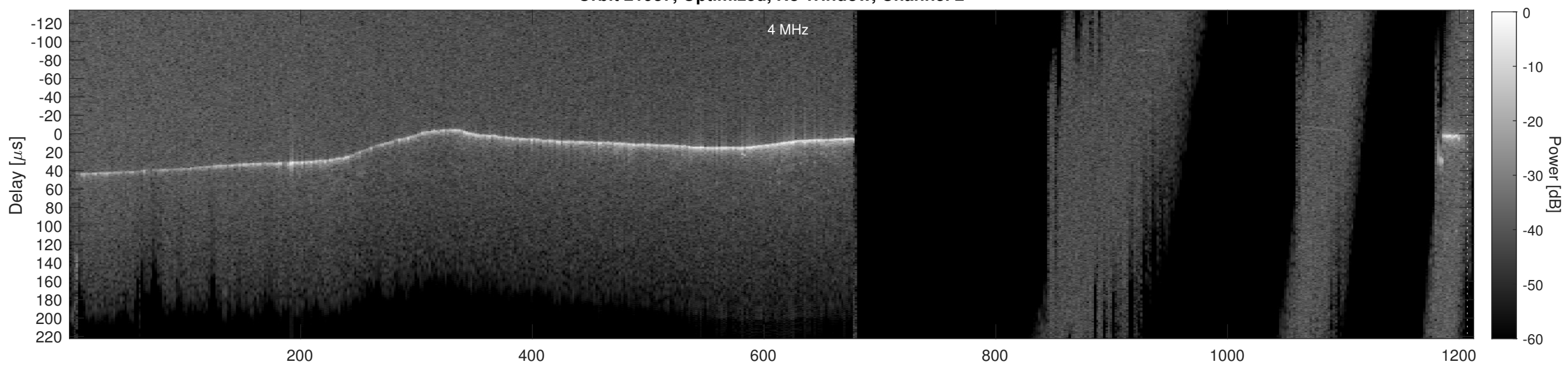
Orbit 21937, Cluttergram
