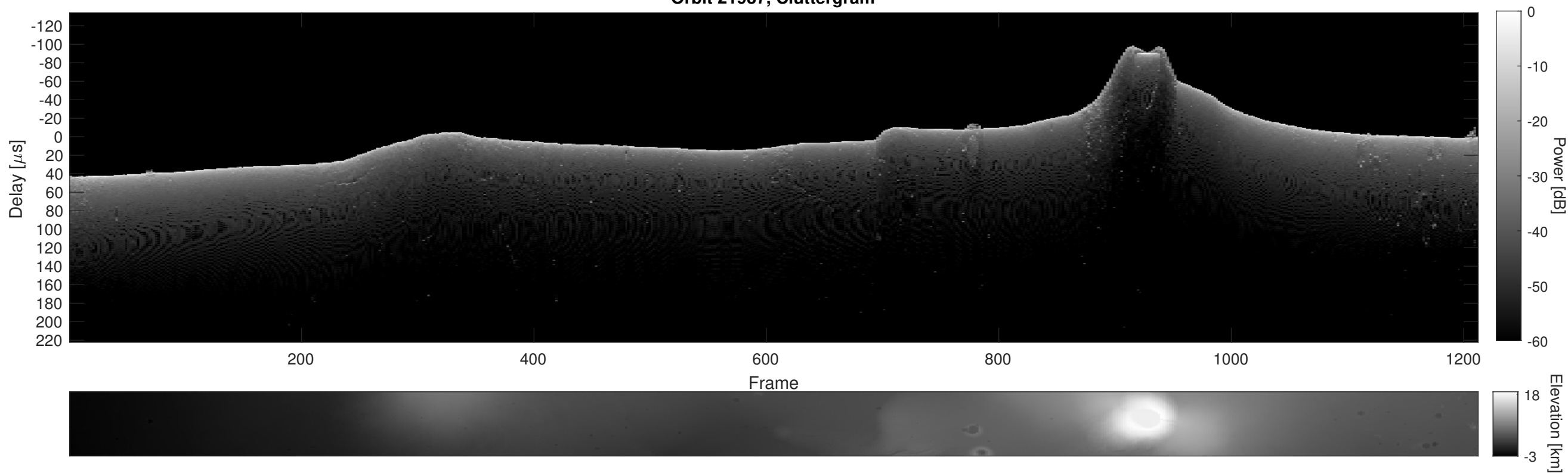
Orbit 21937, Cluttergram
