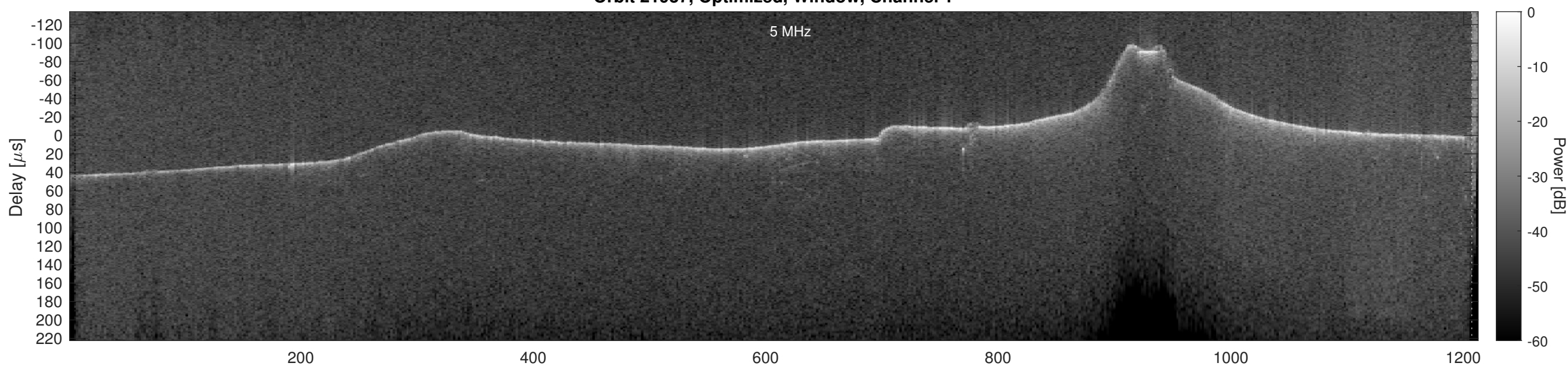
Orbit 21937, Optimized, Window, Channel 2
