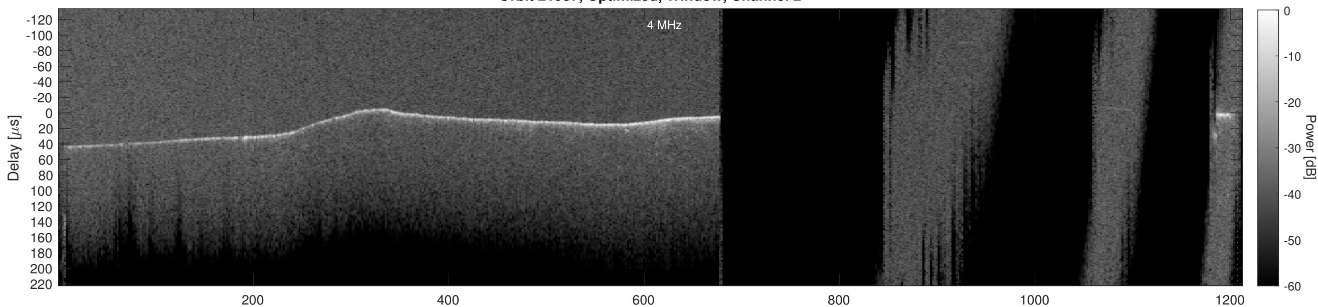
Orbit 21937, Cluttergram
