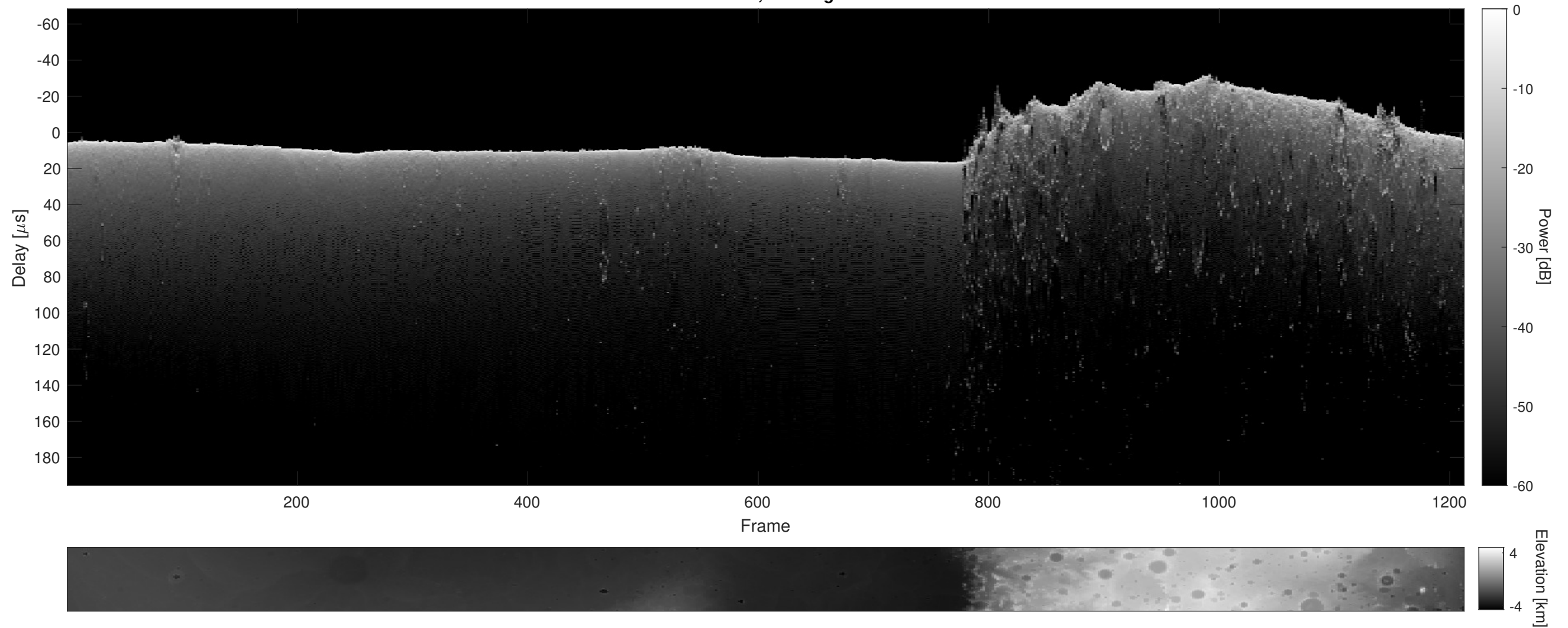
Orbit 21942, Cluttergram
