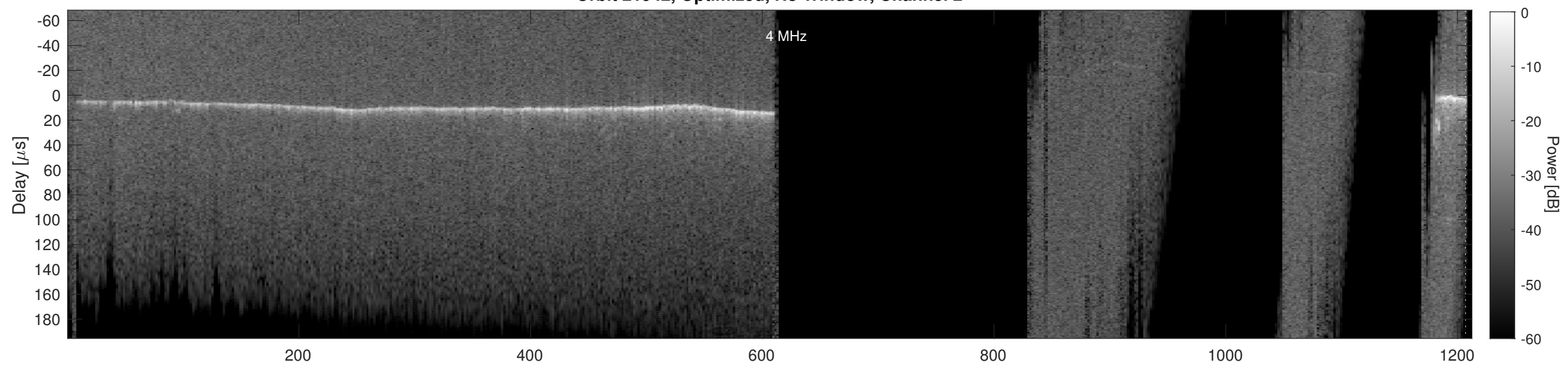
Orbit 21942, Cluttergram
