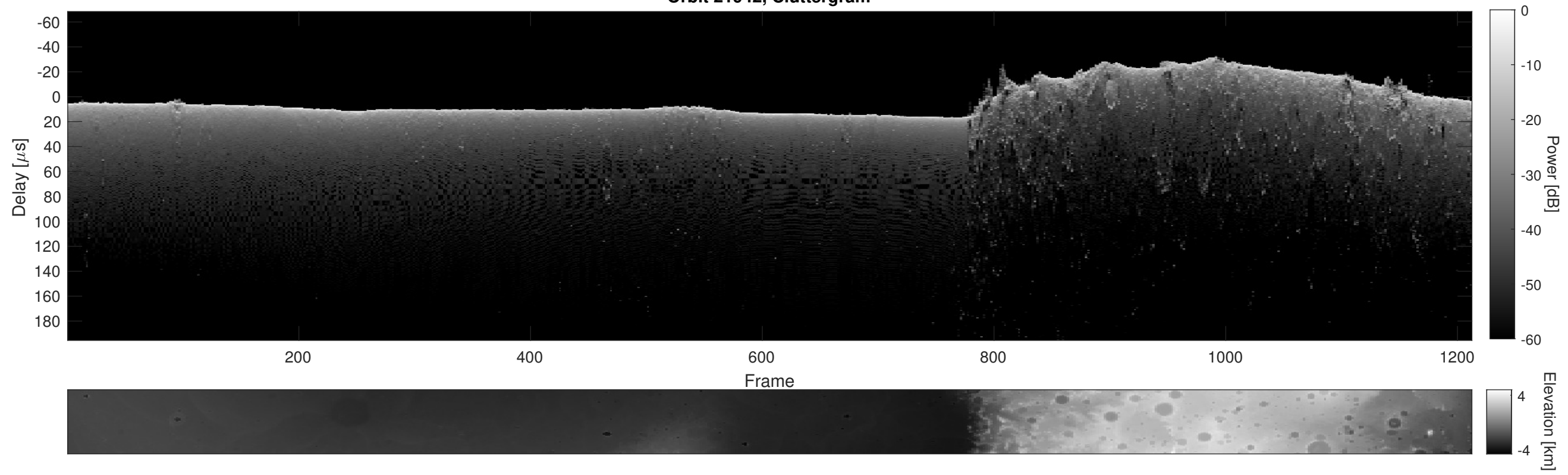
Orbit 21942, Cluttergram
