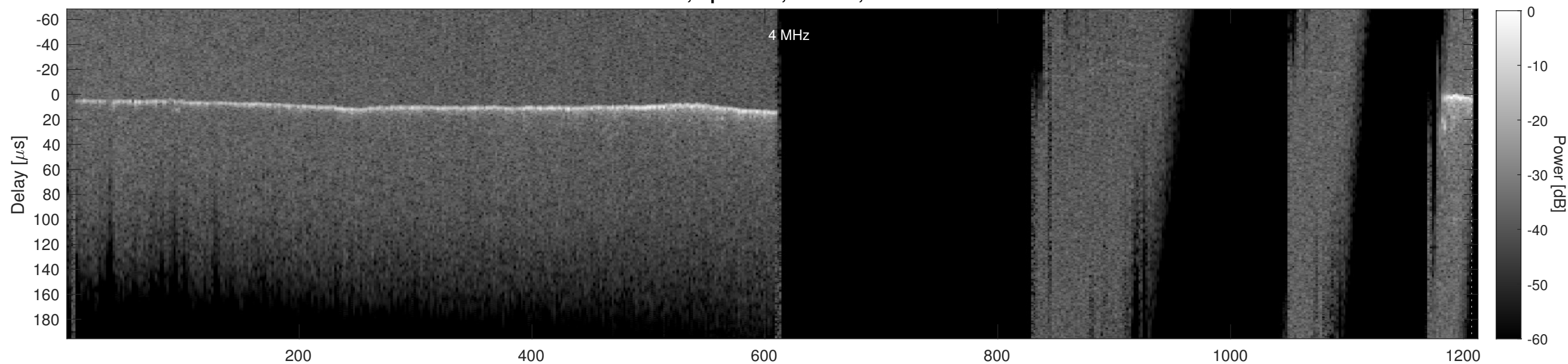
Orbit 21942, Cluttergram
