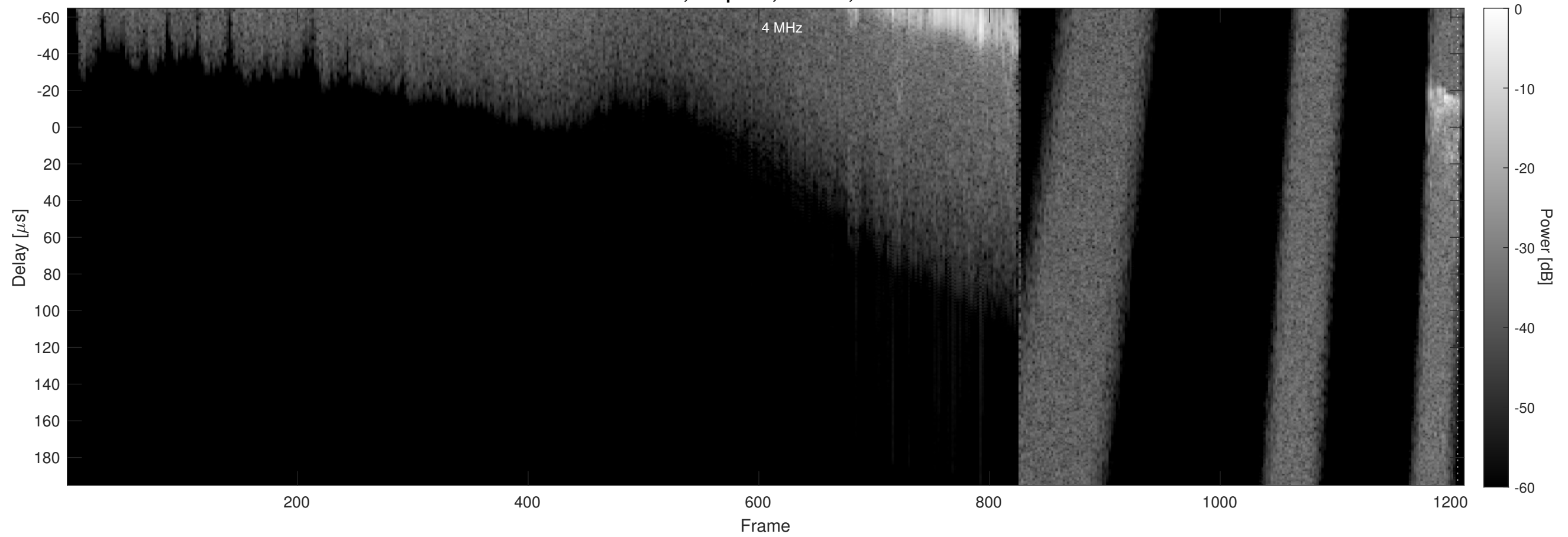
Orbit 21945, Chapman, Window, Channel 2
