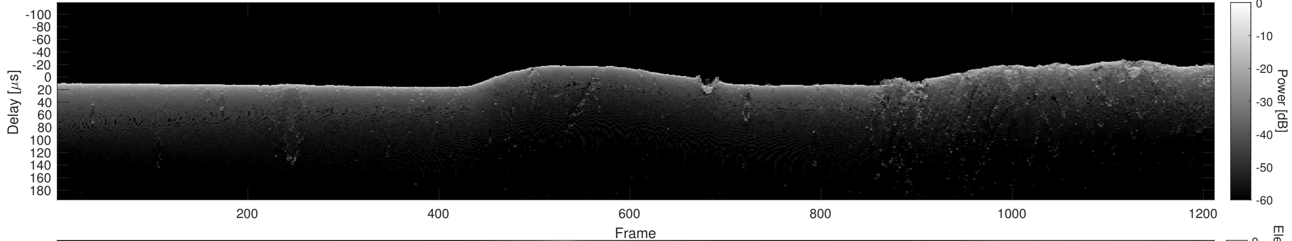
Orbit 21945, Cluttergram
