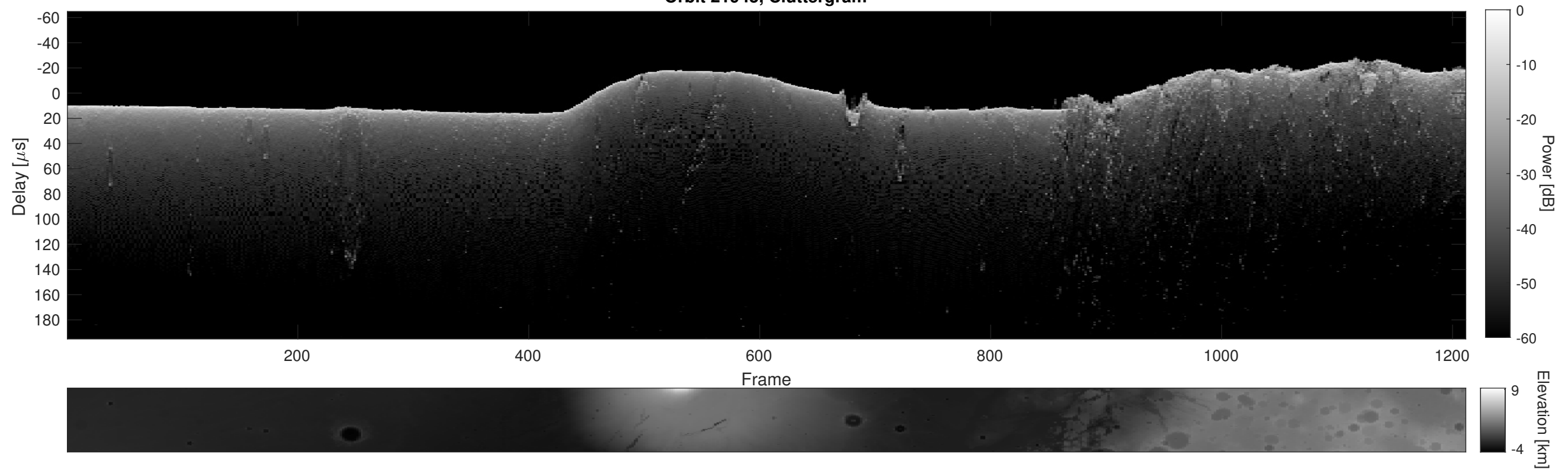
Orbit 21945, Cluttergram
