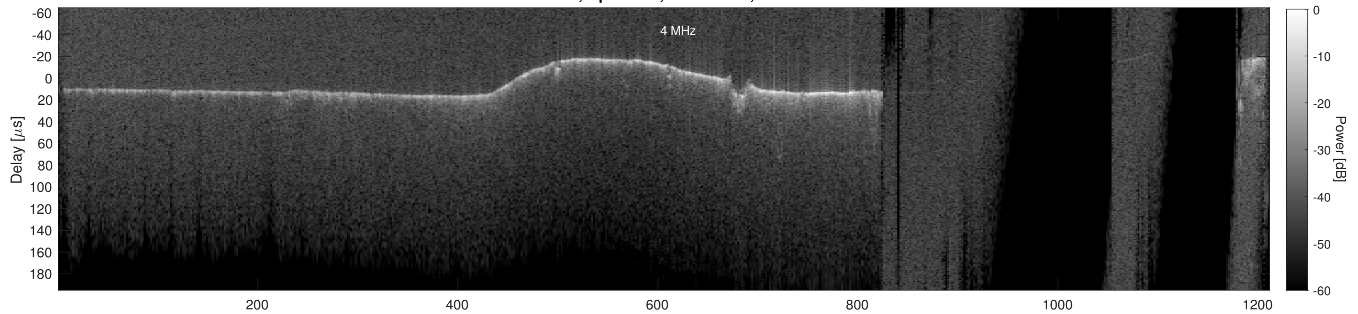
Orbit 21945, Cluttergram
