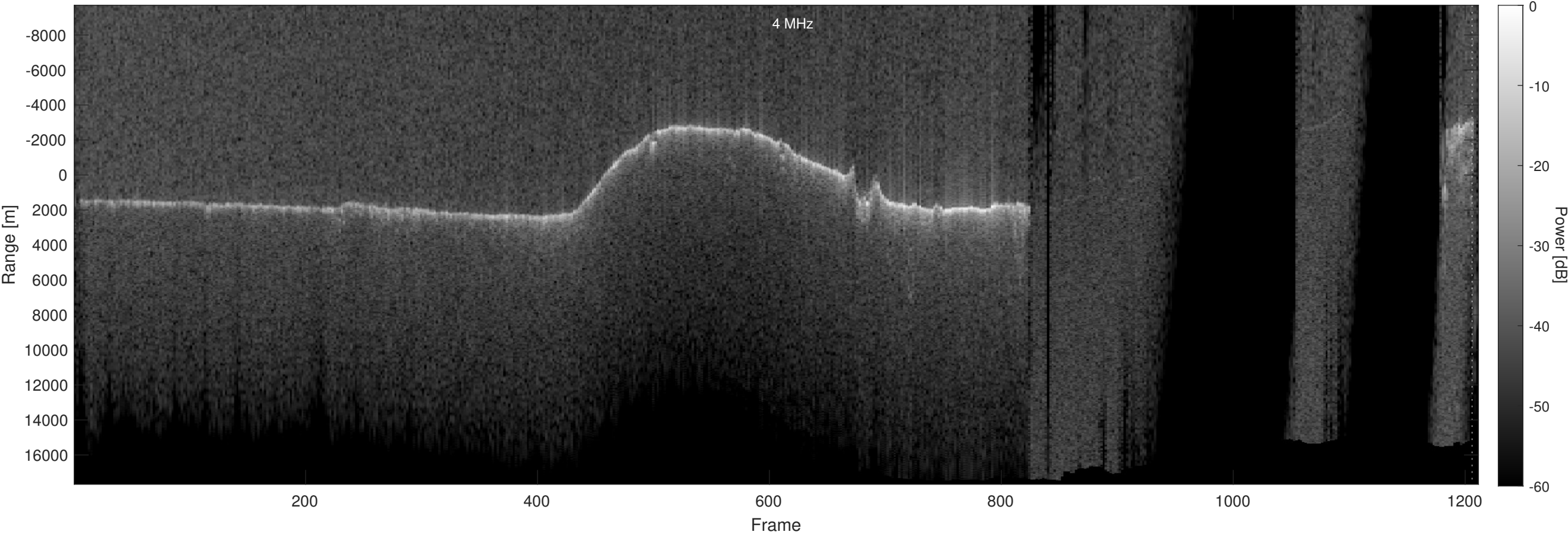
Orbit 21945, Optimized, No Window, Depth-Corrected, Channel 2
