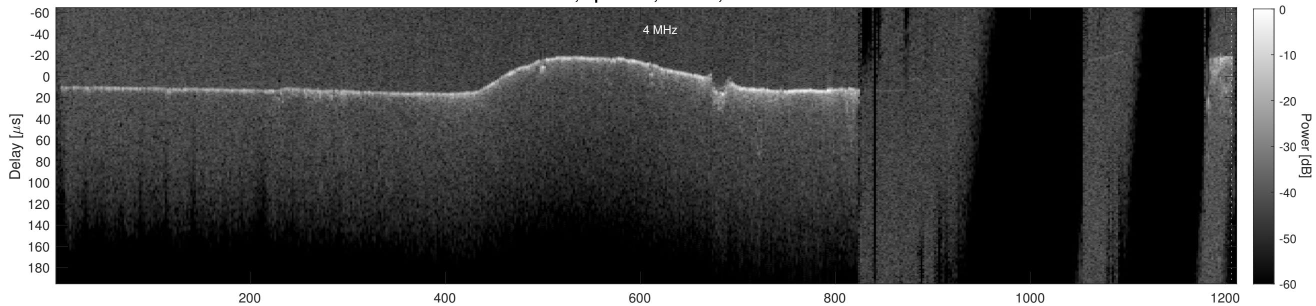
Orbit 21945, Cluttergram
