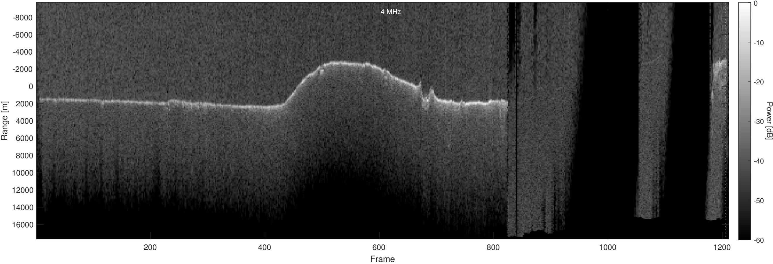
Orbit 21945, Optimized, Window, Depth-Corrected, Channel 2
