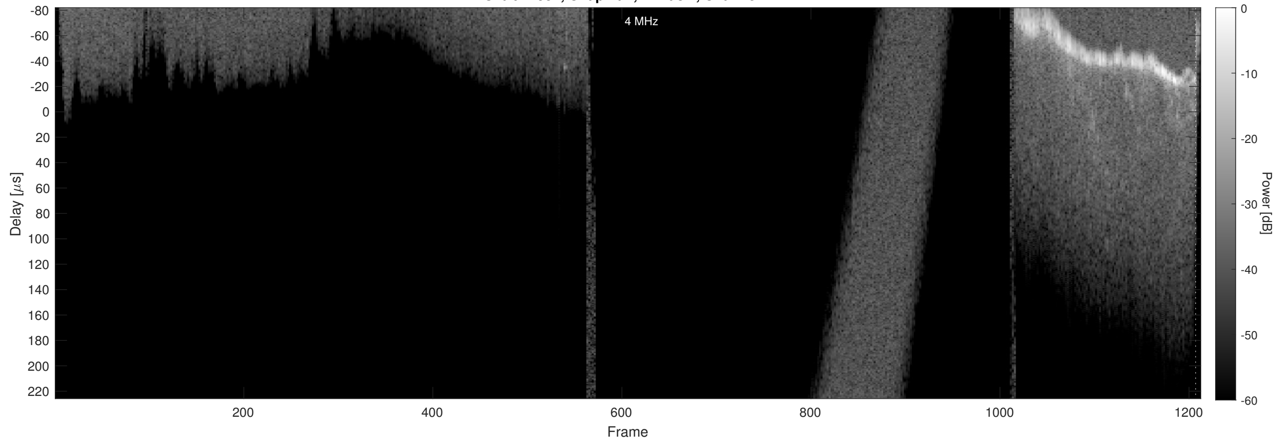
Orbit 21951, Chapman, Window, Channel 2
