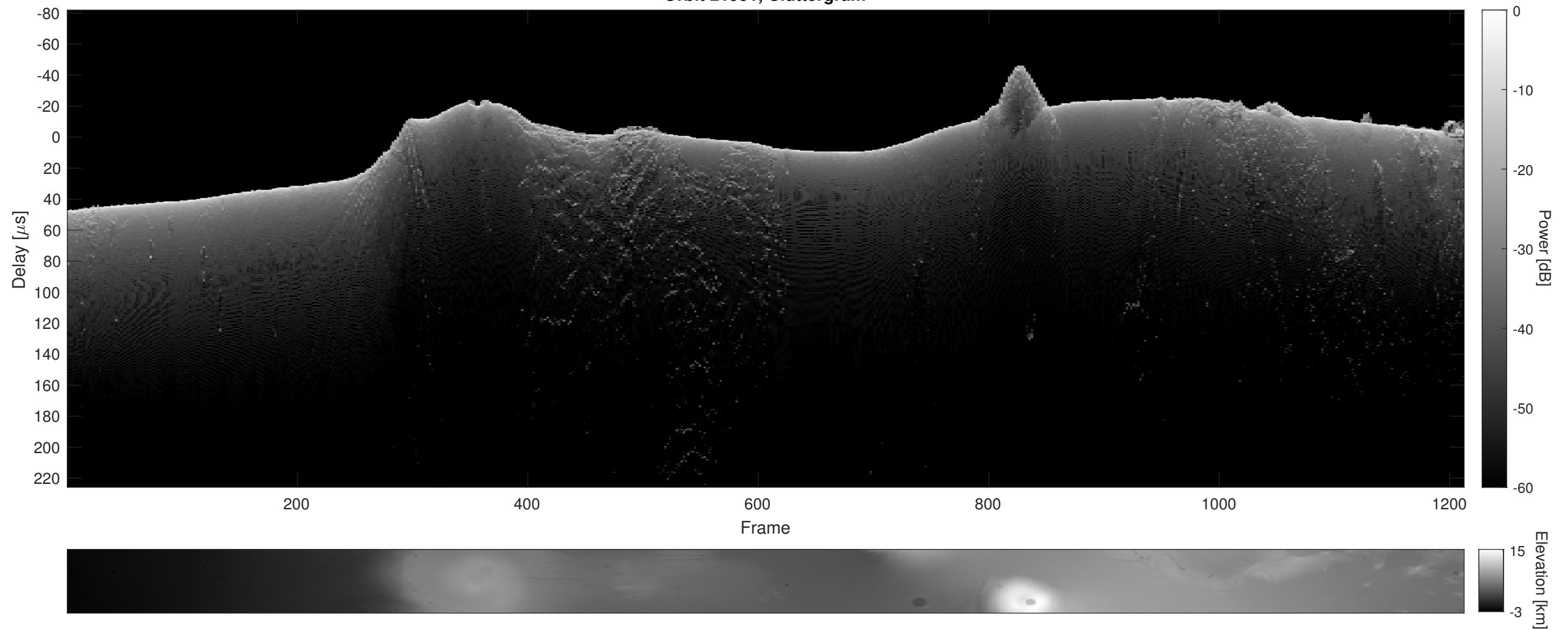
Orbit 21951, Cluttergram
