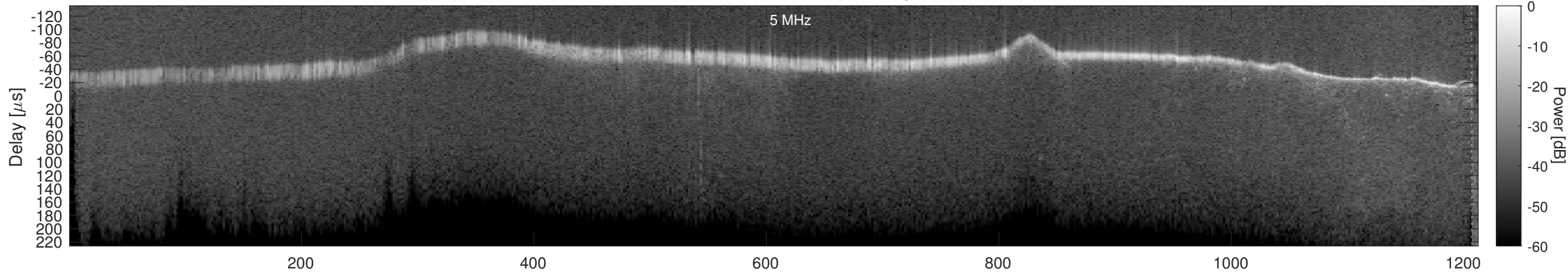
Orbit 21951, Window, Channel 1, Optimized
