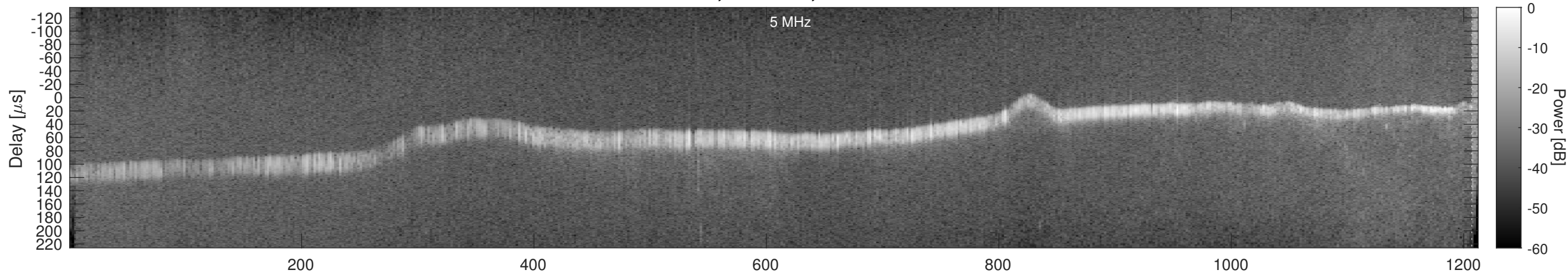
Orbit 21951, Window, Channel 1, Chapman
