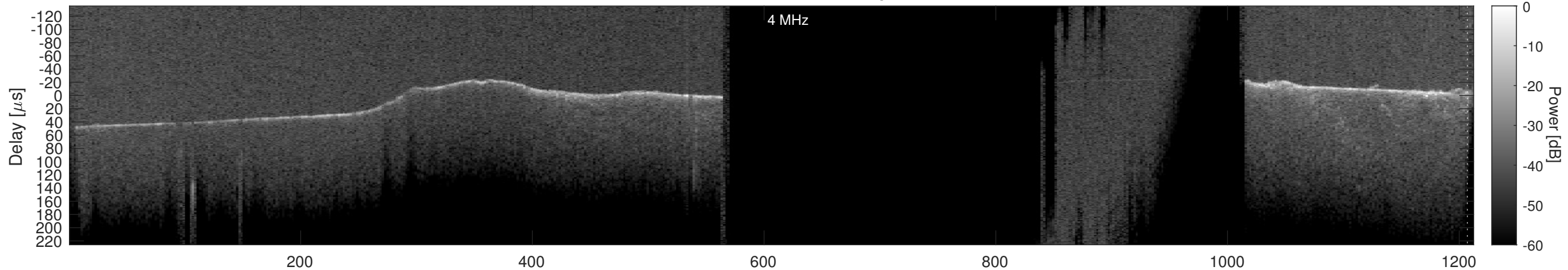
Orbit 21951, Cluttergram
