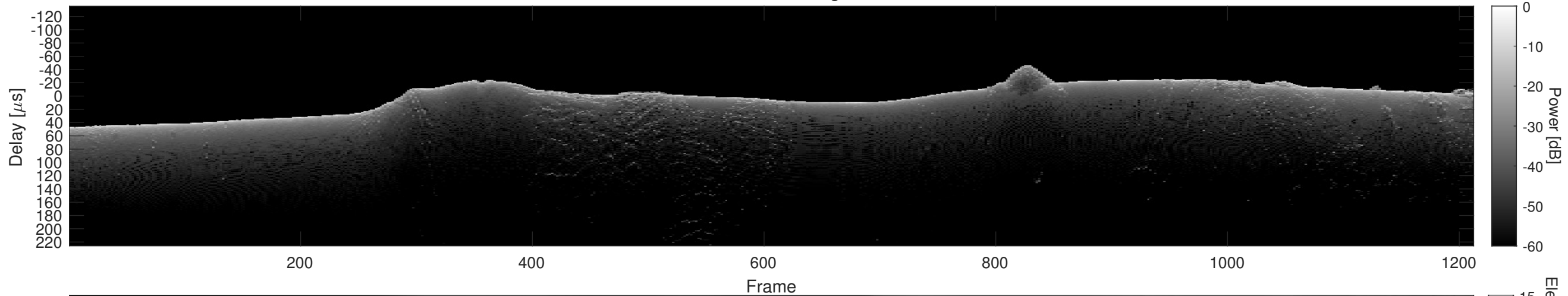
Orbit 21951, Cluttergram
