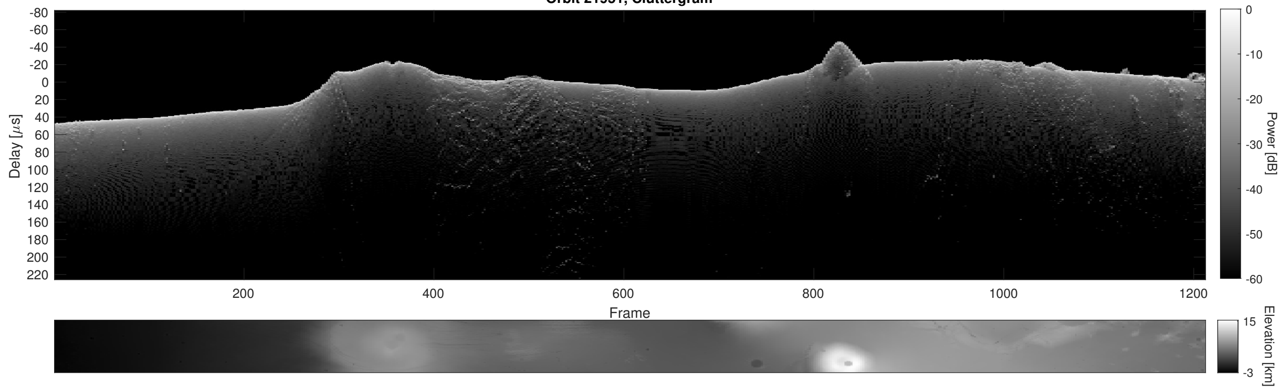
Orbit 21951, Cluttergram
