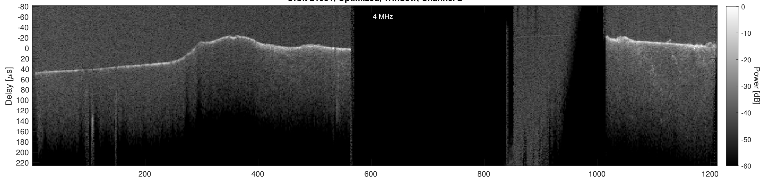
Orbit 21951, Cluttergram
