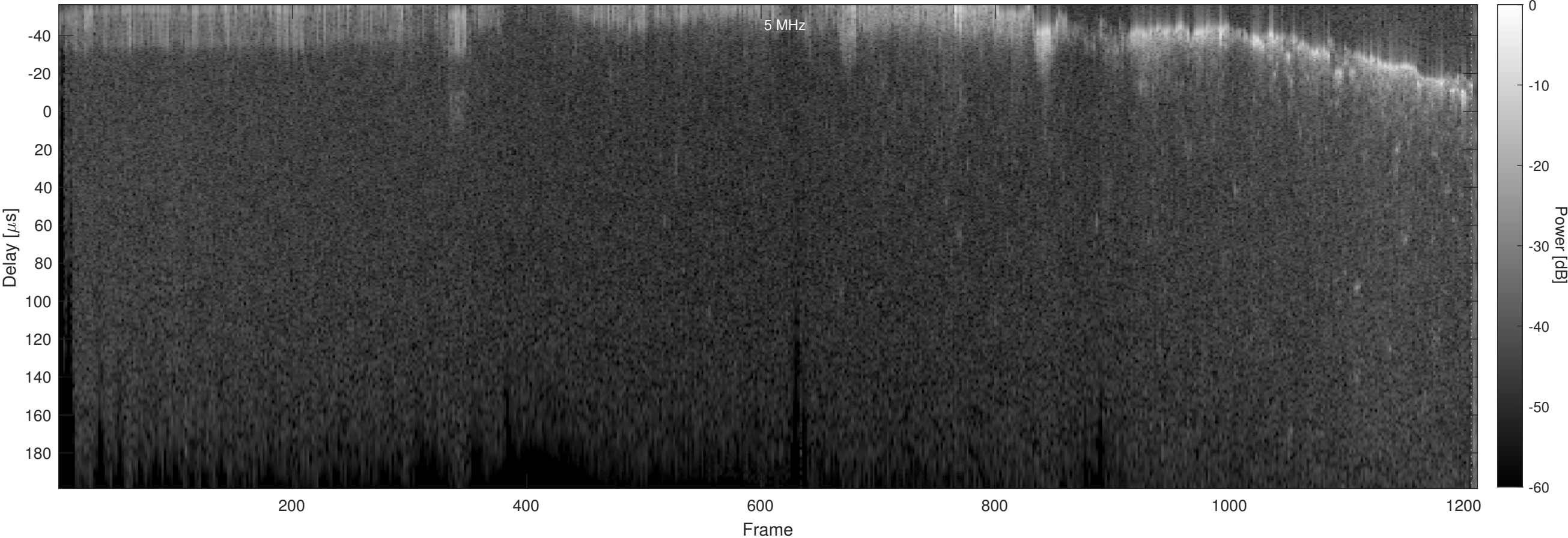
Orbit 21953, Chapman, No Window, Channel 2
