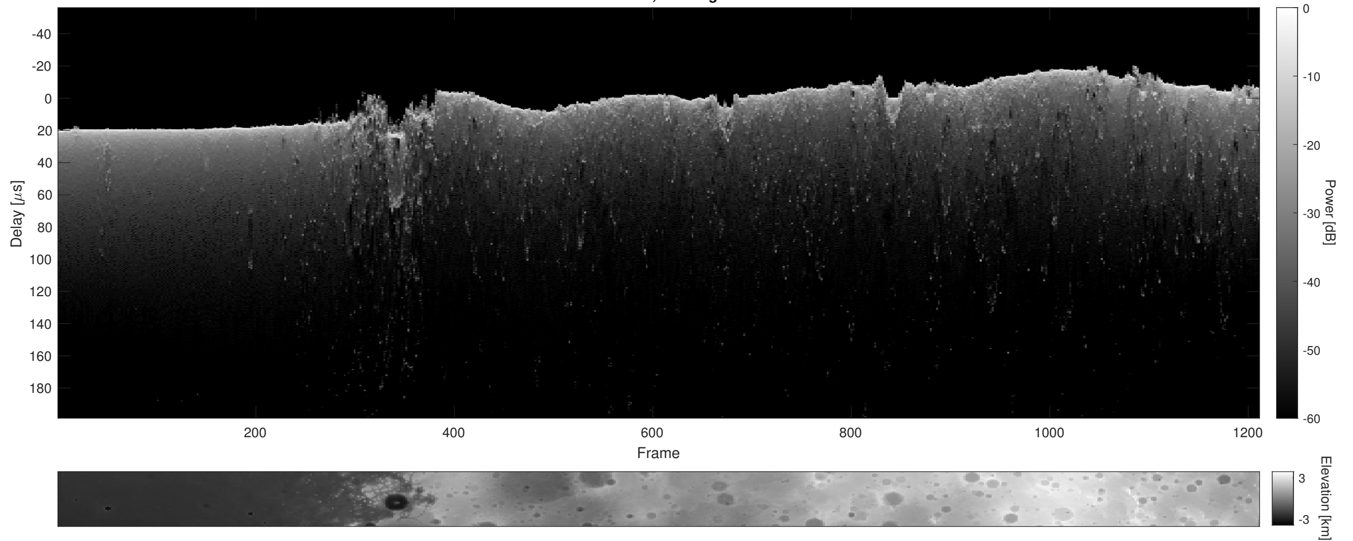
Orbit 21953, Cluttergram
