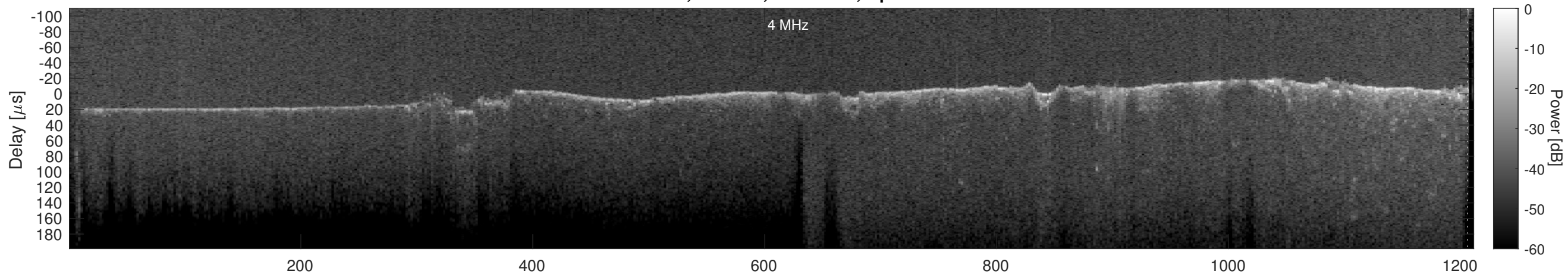
Orbit 21953, Cluttergram
