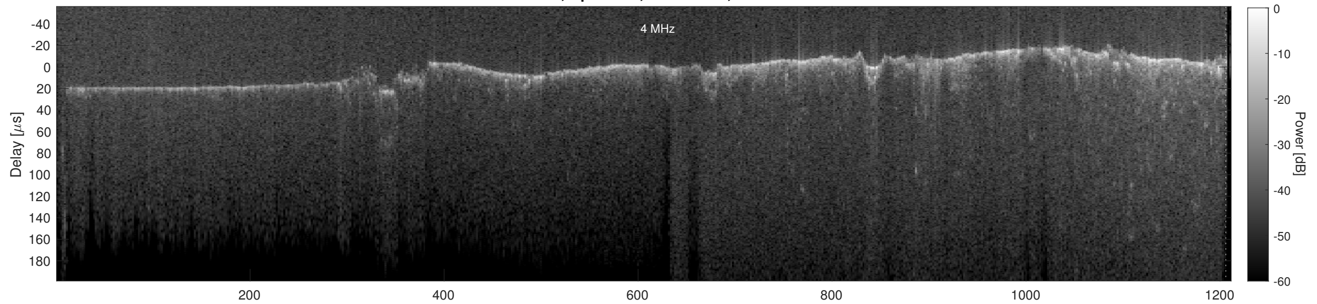
Orbit 21953, Cluttergram
