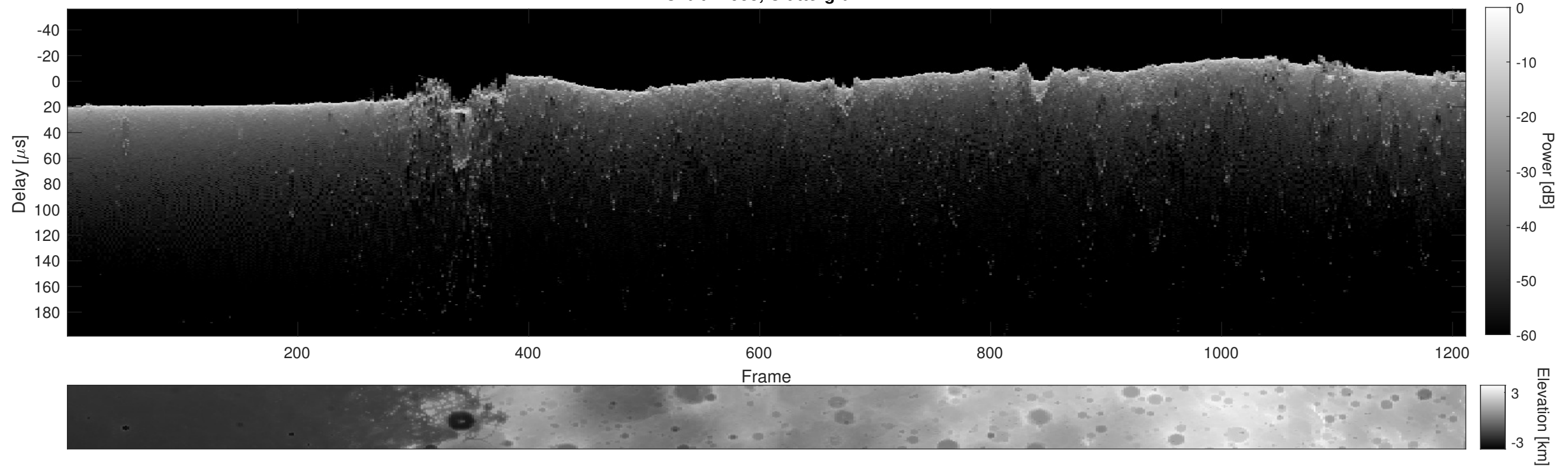
Orbit 21953, Cluttergram
