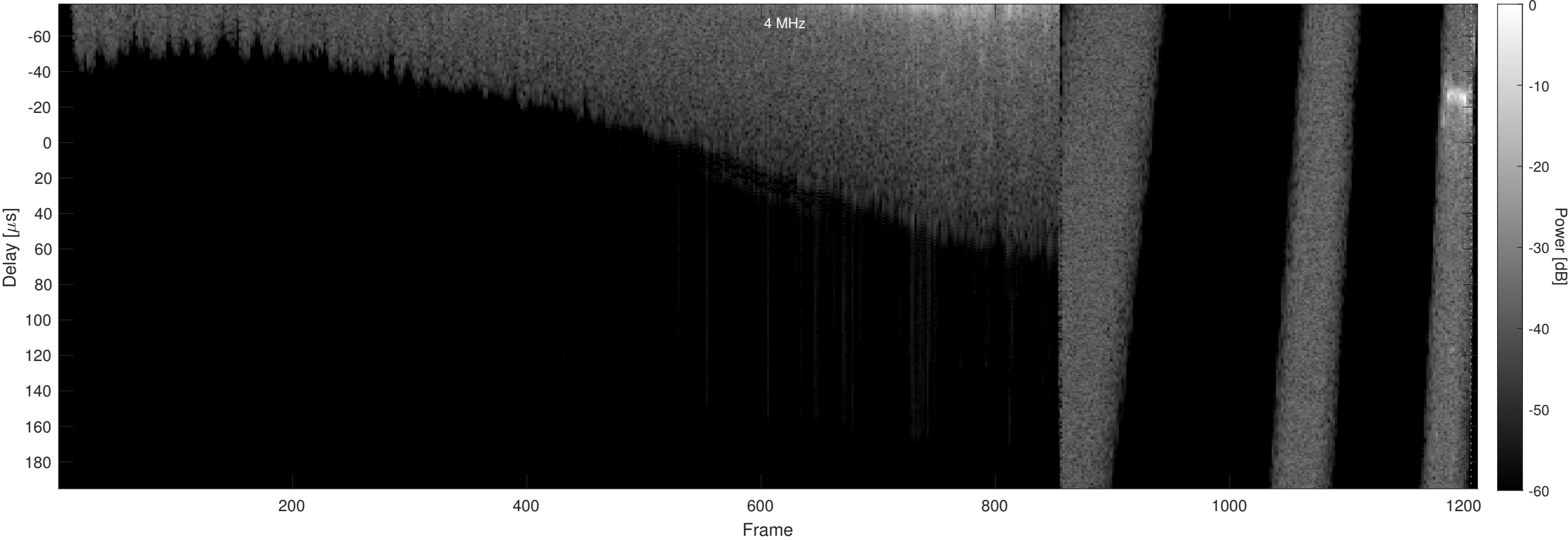
Orbit 21956, Chapman, No Window, Channel 2
