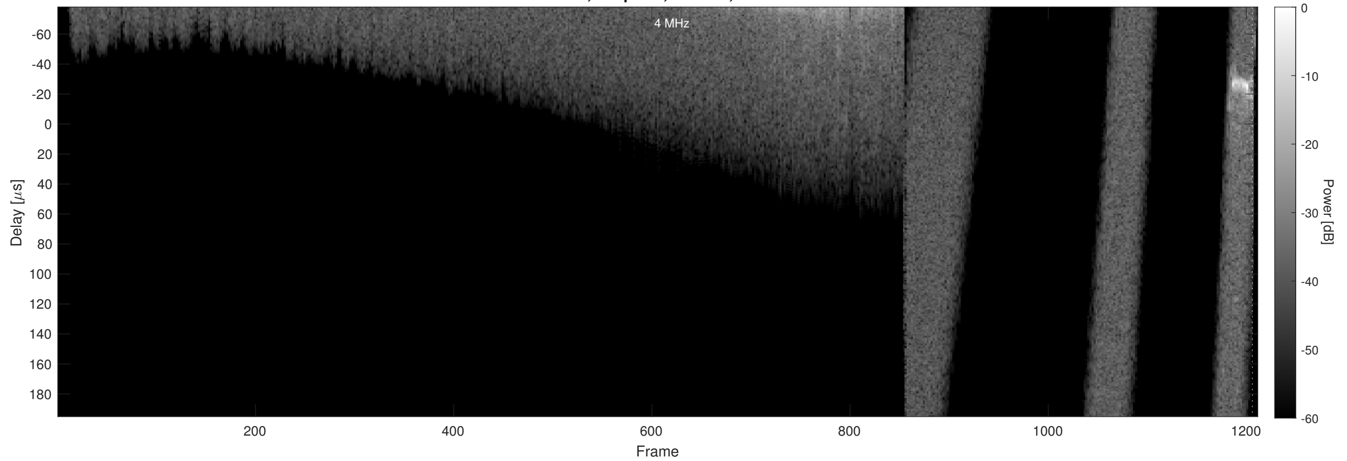
Orbit 21956, Chapman, Window, Channel 2
