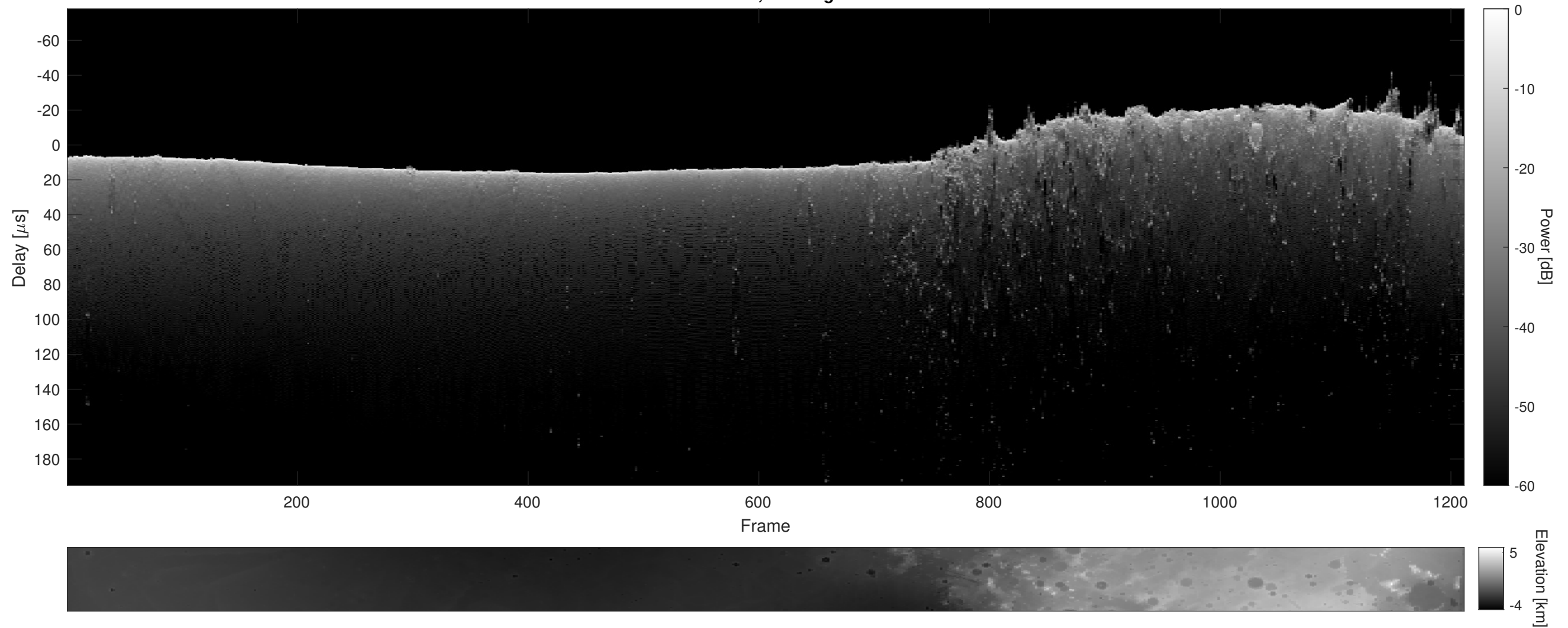
Orbit 21956, Cluttergram
