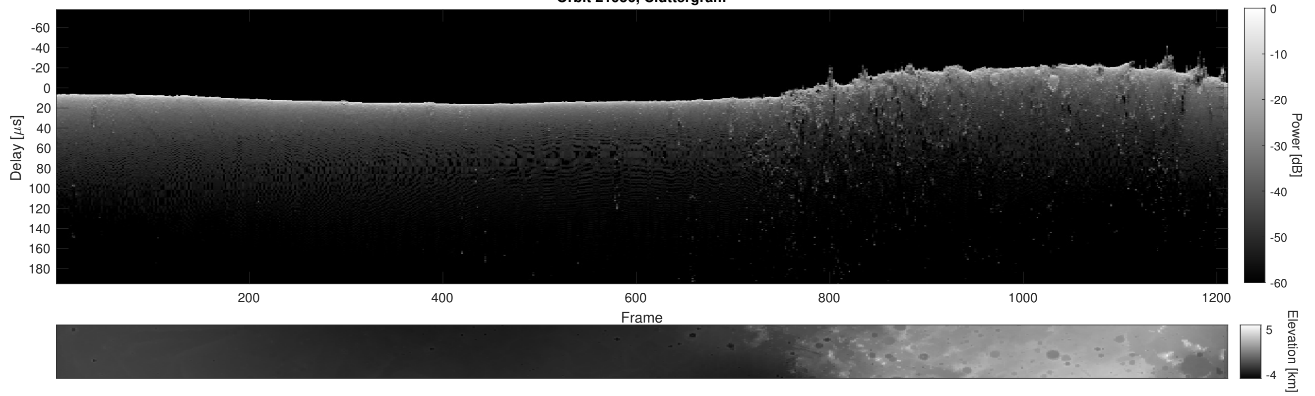
Orbit 21956, Cluttergram
