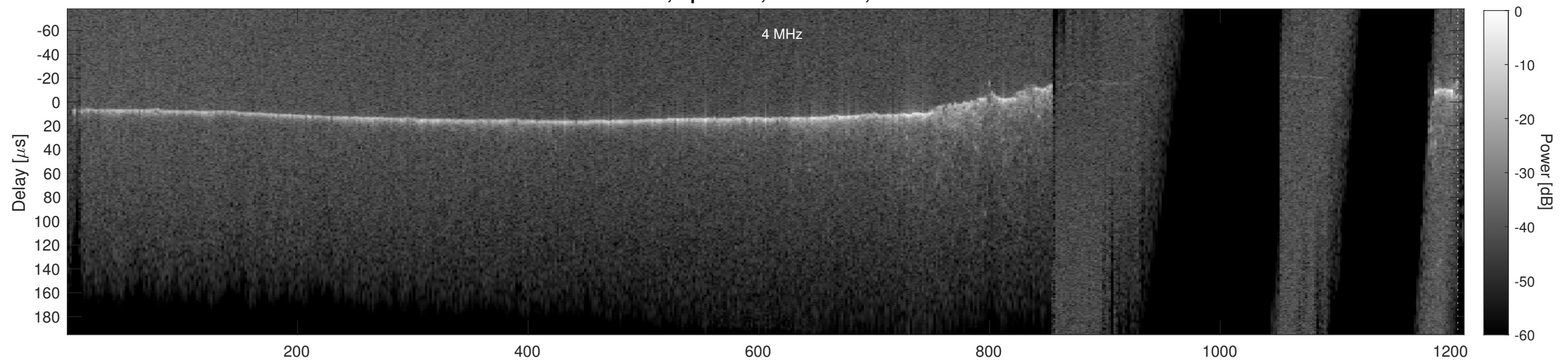
Orbit 21956, Cluttergram
