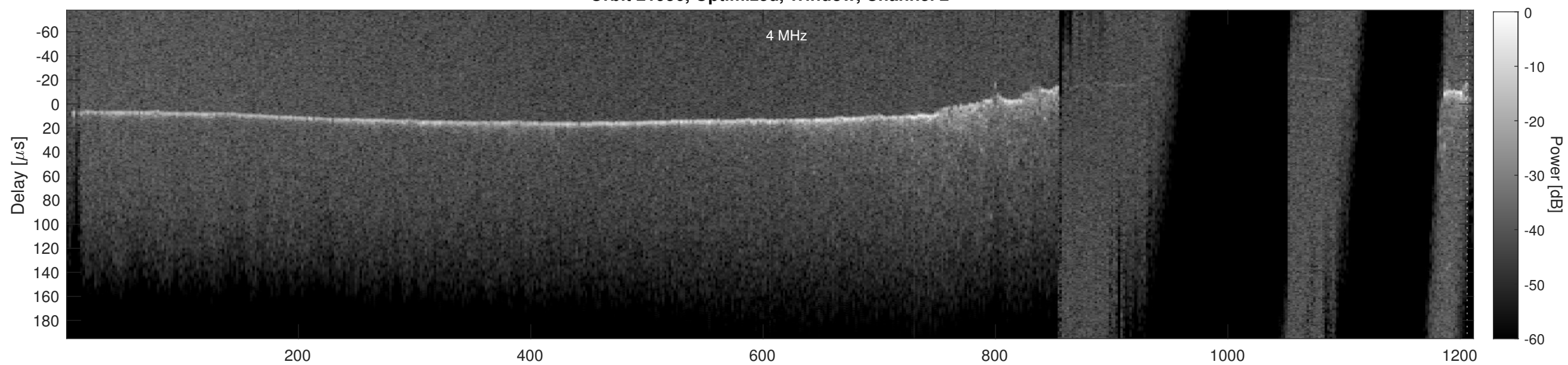
Orbit 21956, Cluttergram
