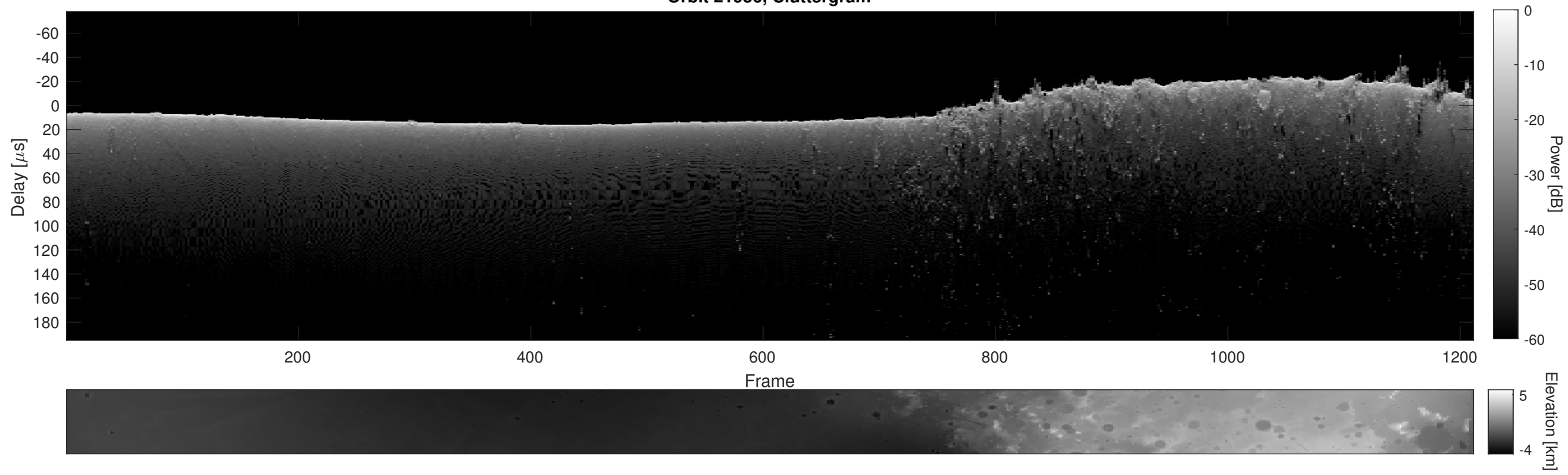
Orbit 21956, Cluttergram
