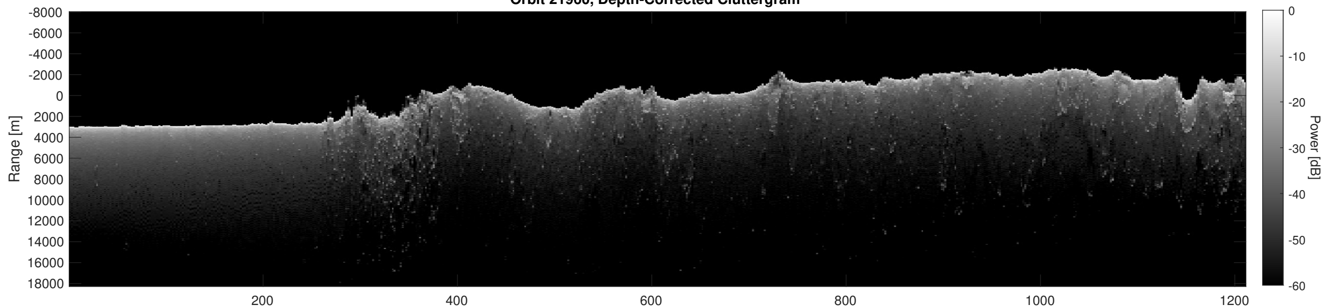
Orbit 21960, Depth-Corrected Cluttergram
